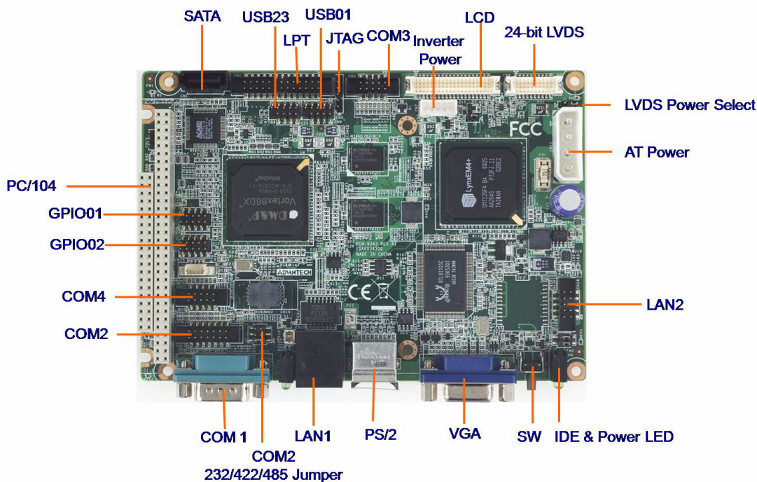
Figure 2.1 Jumper and Connector layout (Component side)
