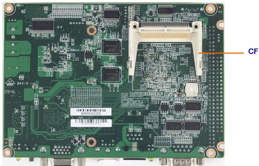
Figure 2.2 Jumper and Connector layout (Solder side)
