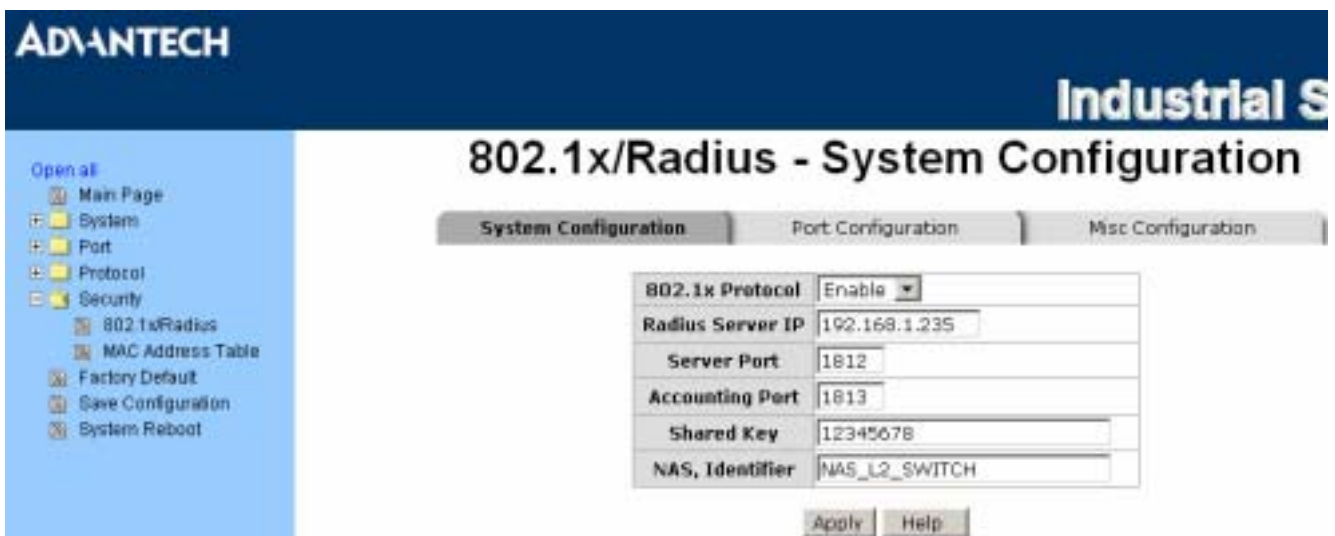
Figure 3.49: 802.1x/RADIUS System Configuration interface
