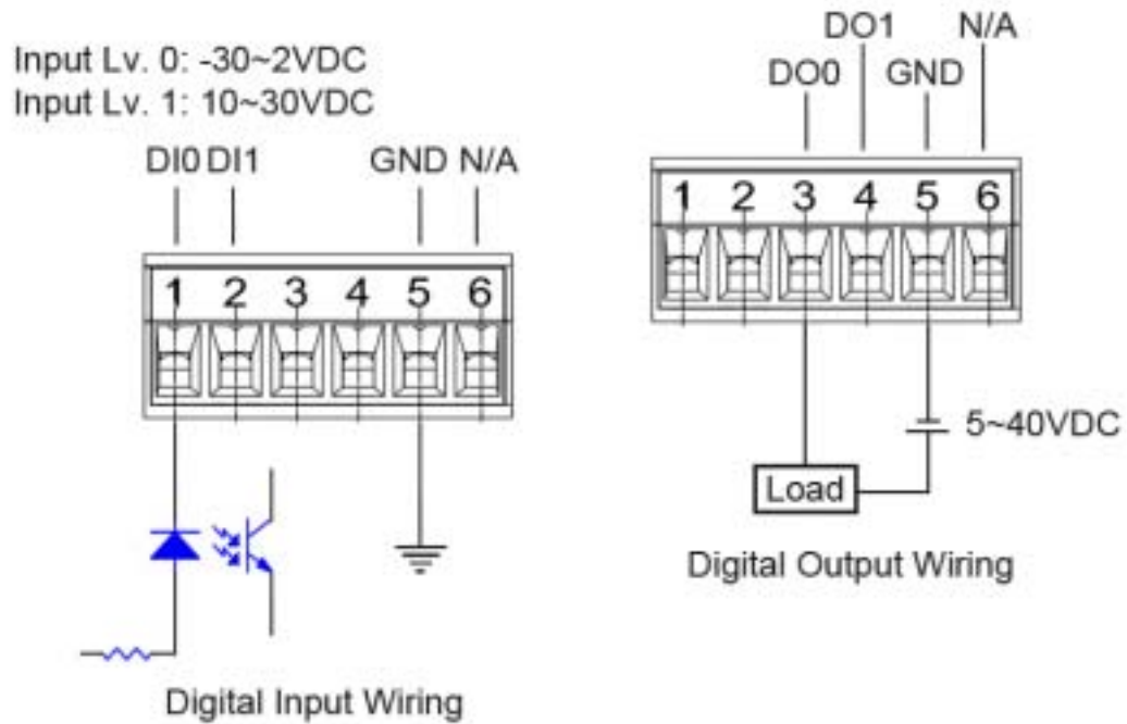
Figure 2.14: Pin Assignment of the DIDO Connector
