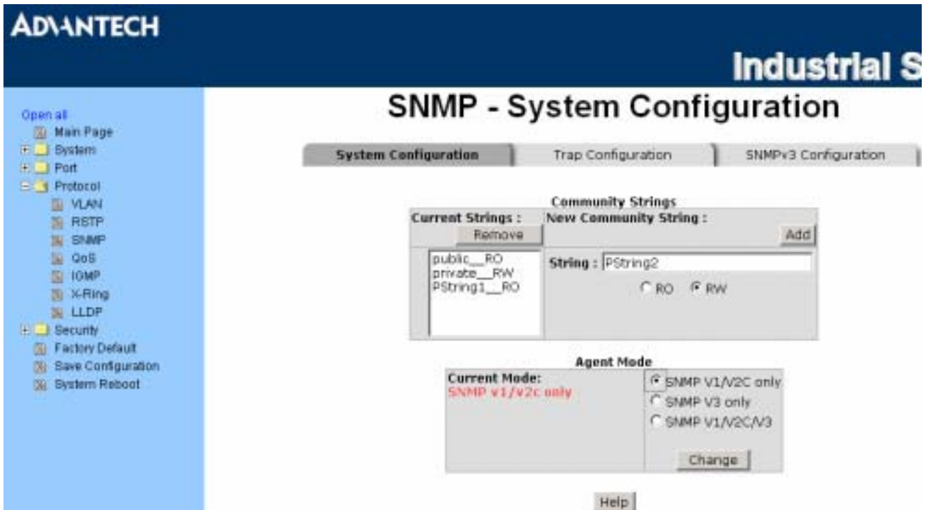
Figure 3.42: SNMP System Configuration interface
