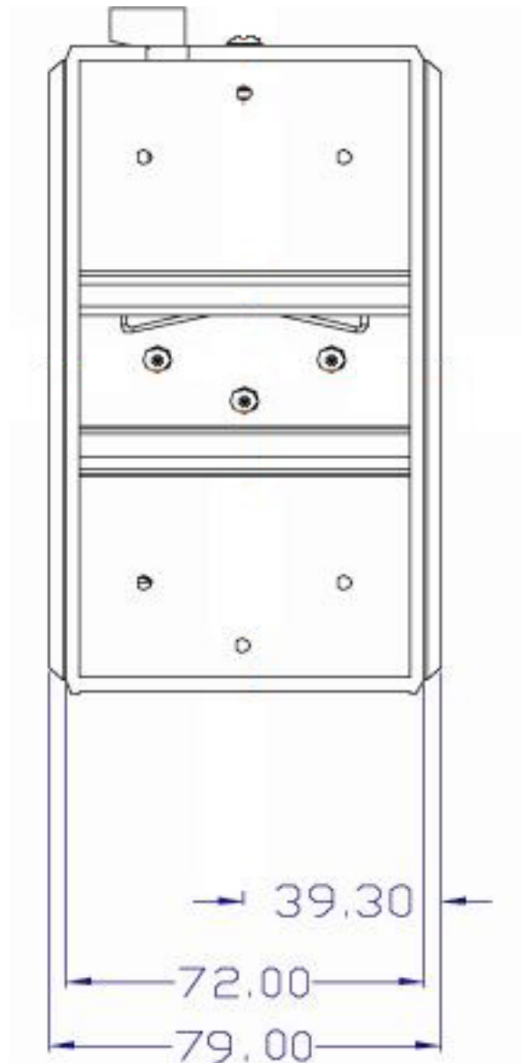
Figure 2.3: Rear View of EKI-7657C
