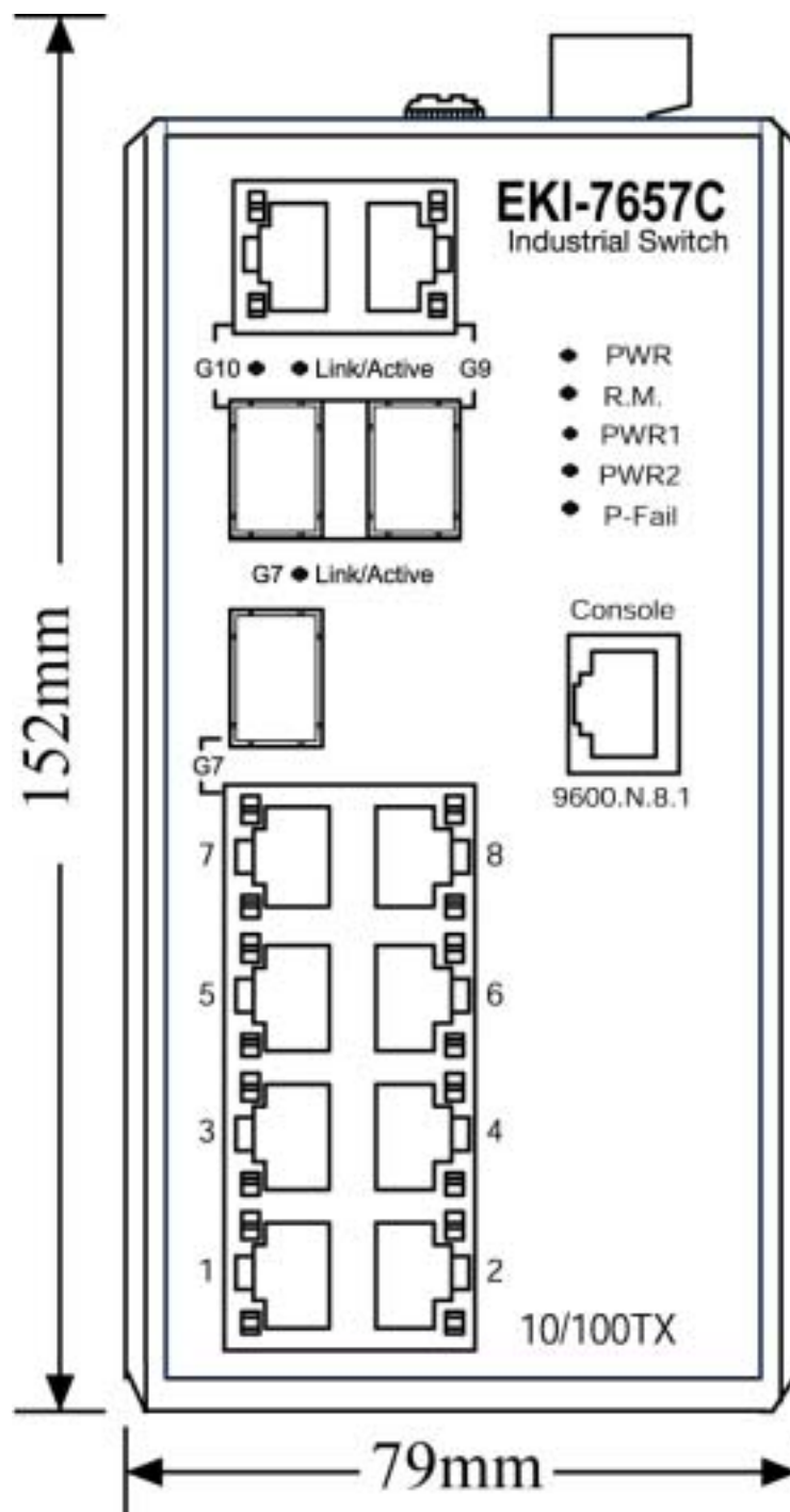
Figure 2.1: Front View of EKI-7657C
