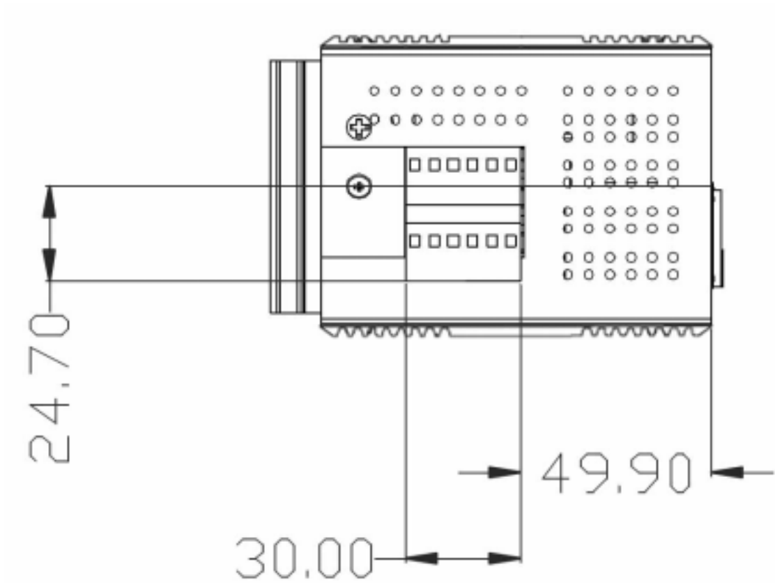
Figure 2.4: Top View of EKI-7657C
