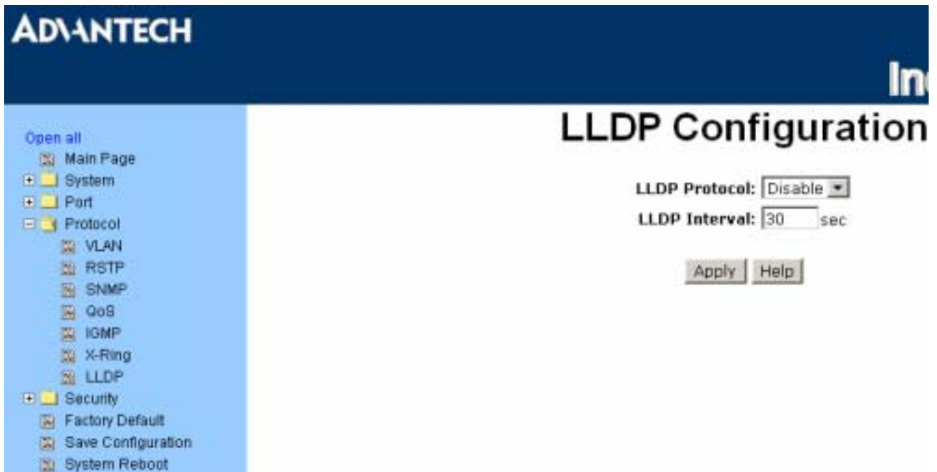
Figure 3.48: LLDP Configuration interface
