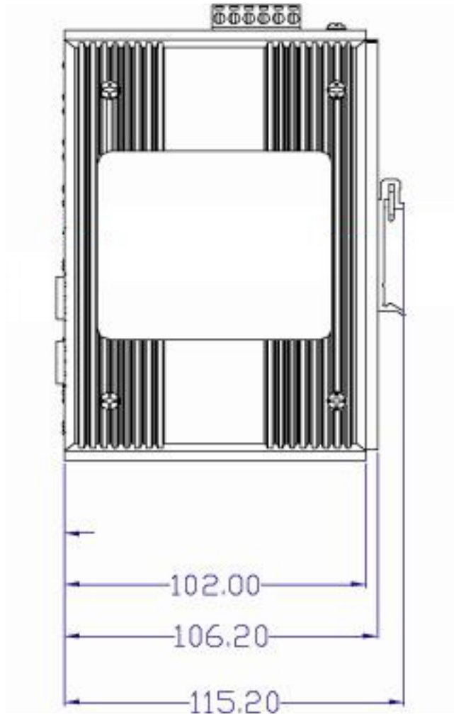
Figure 2.2: Side View of EKI-7657C
