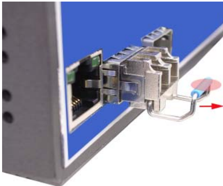
Figure 2.12: Pull out from the transceiver
