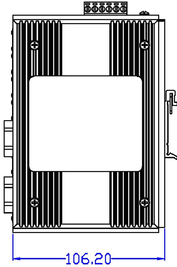
Figure 2.2: Side View of EKI-7526MI
