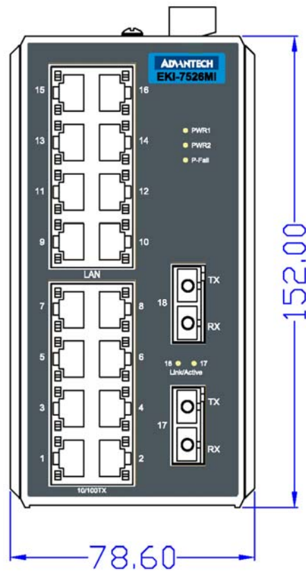
Figure 2.1: Front View of EKI-7526MI
