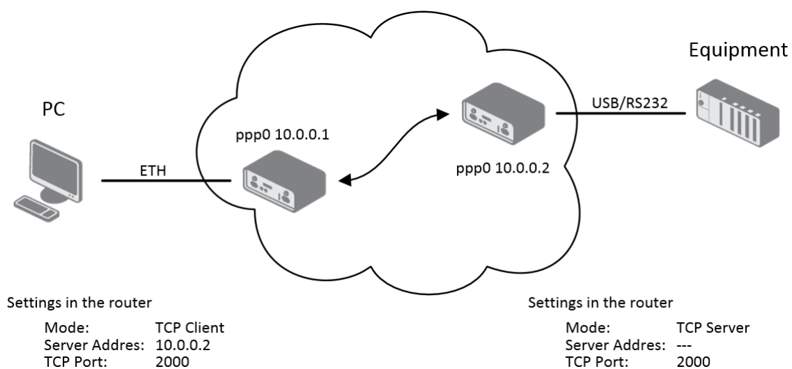
Figure 64: Example 2 – USB port configuration
