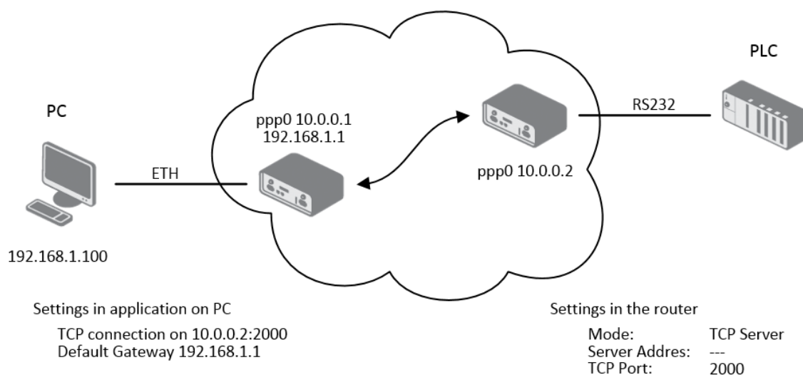
Figure 60: Example of Ethernet to serial communication
