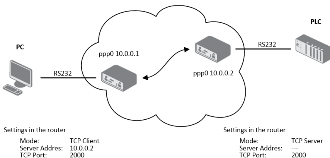
Figure 61: Example of serial port extension
