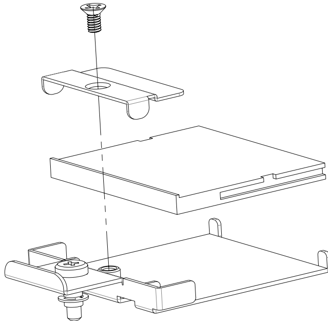
Figure 3.2 Installing the Compact Flash card
