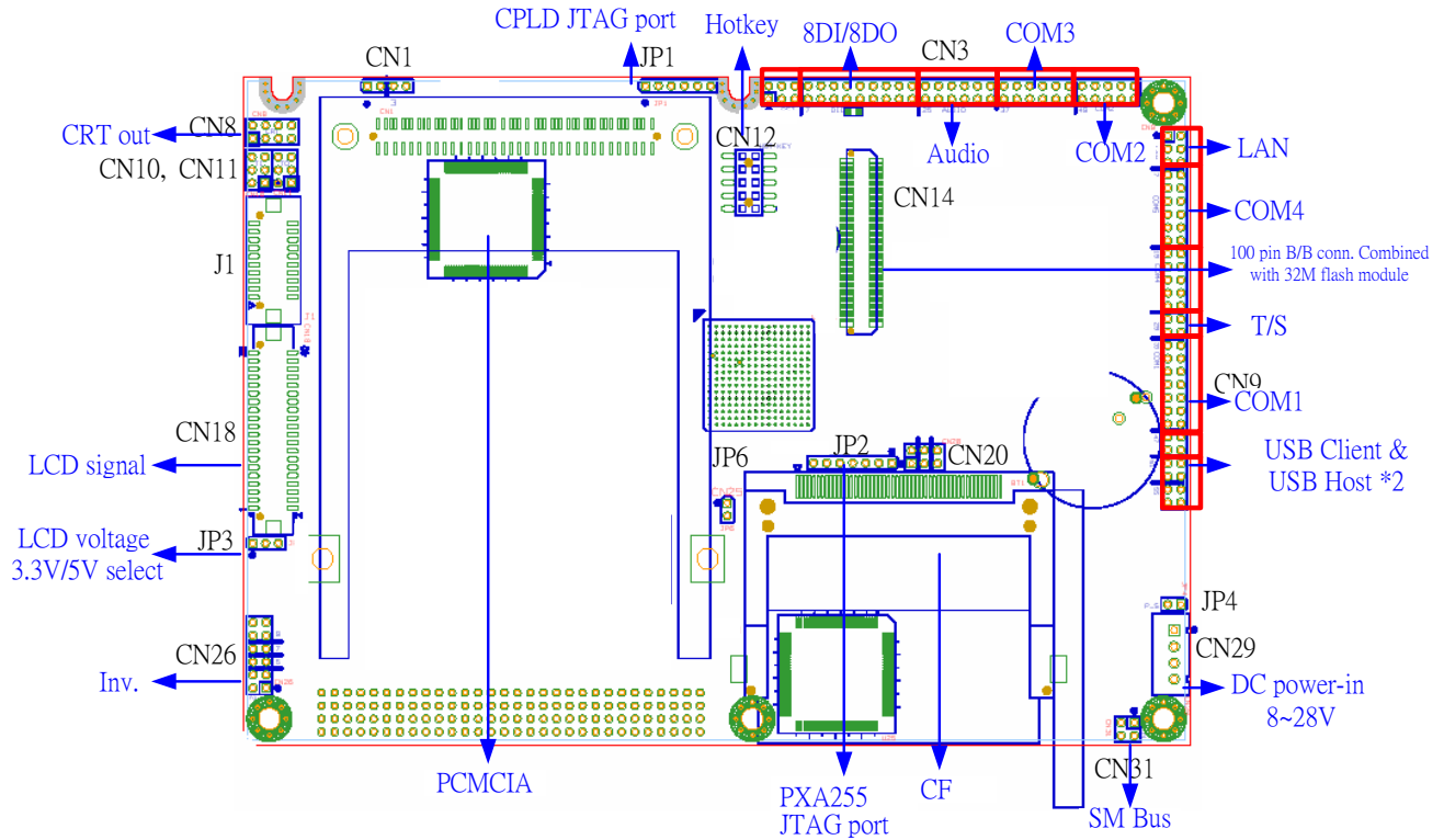
Figure 3.2: Component side of the PCM-7230
