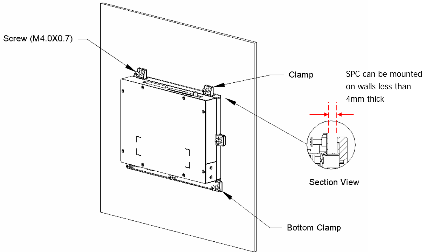
Rear View (SPC-64A)
