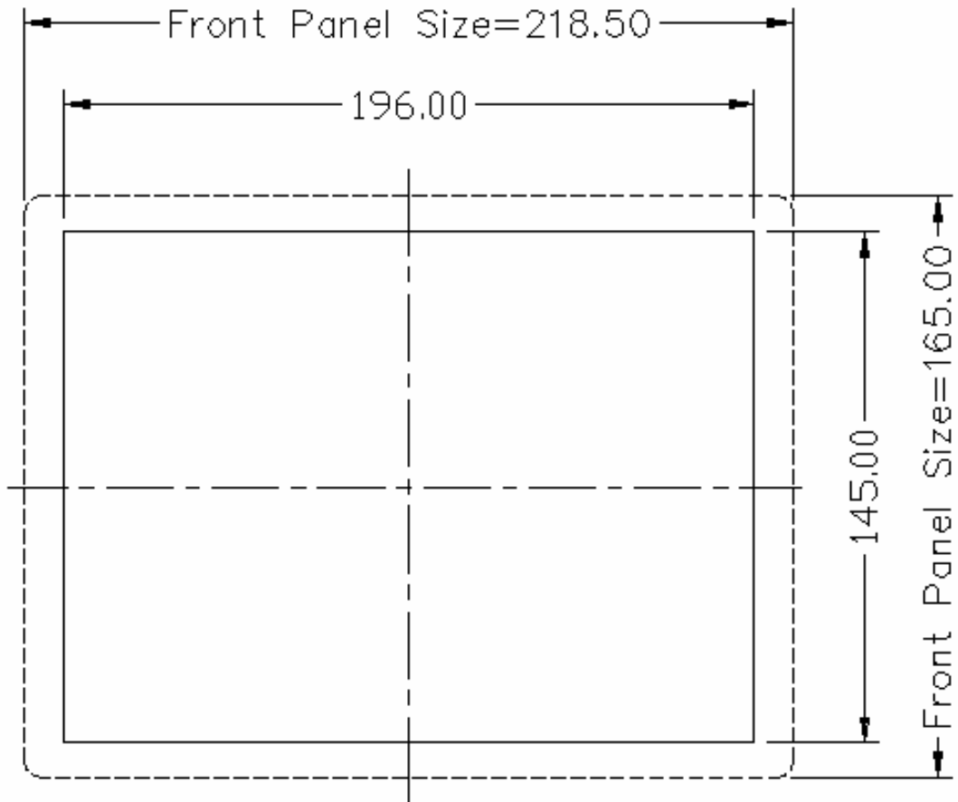
Front View for Panel Mount (SPC-64A)
