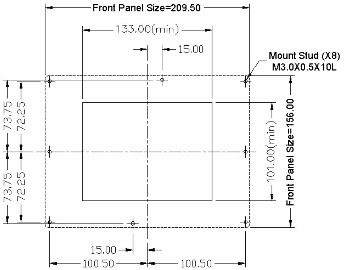
Front View for Panel Mount (SPC-64C)
