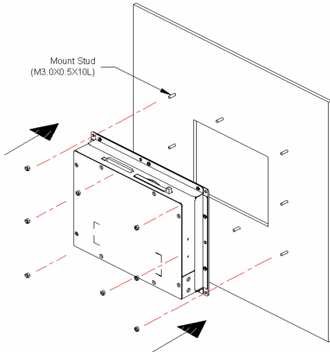
Rear View for Panel Mount (SPC-64C)
