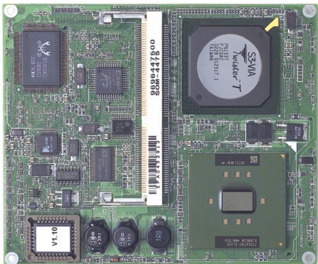
Figure 1-2: SOM-4475 Top view
