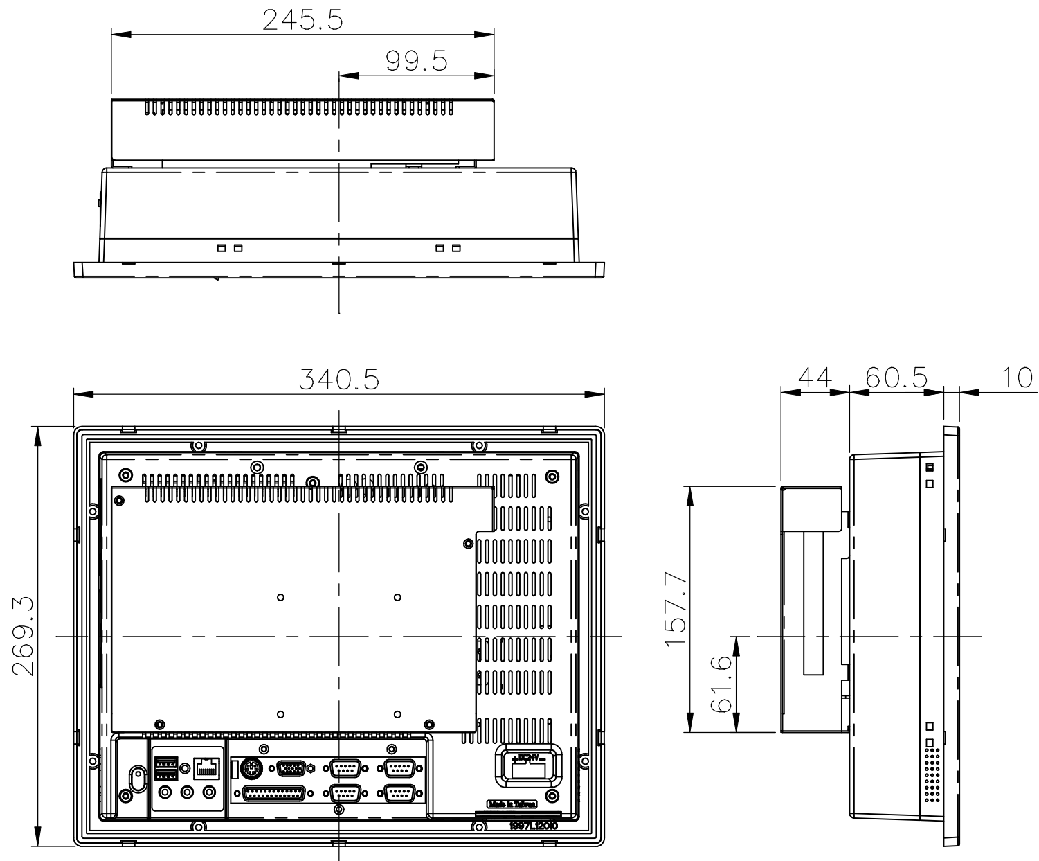
PPC-L126 W/Ext. Box
