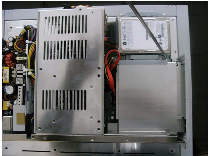
Figure 4.12 Rear Cover Photo with ODD Bracket
