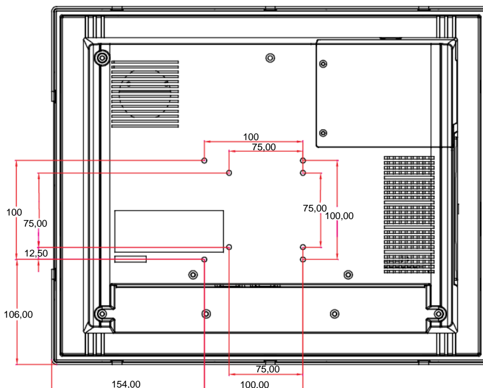
Figure 2.4 Rear View of the Panel PC
