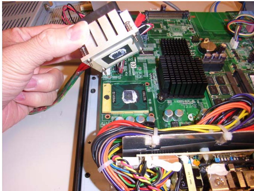
Figure 4.7 Placing the CPU in the Socket
