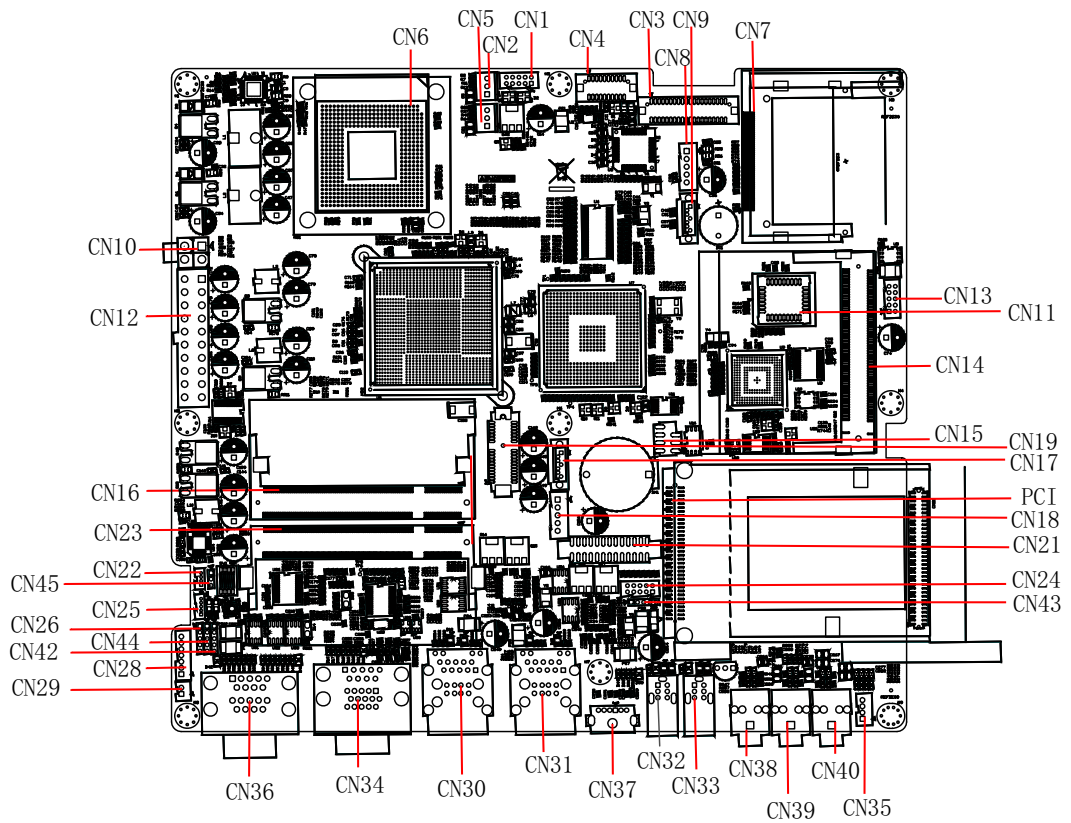
Figure 5.1 Jumpers & Connectors on PPC-177T Motherboard
