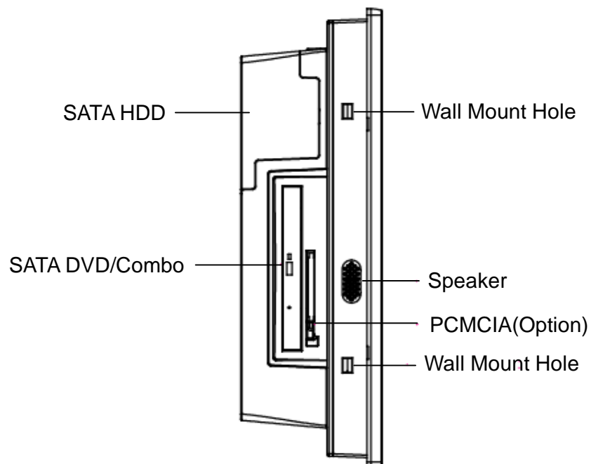
Figure 2.2 Side View of the Panel PC
