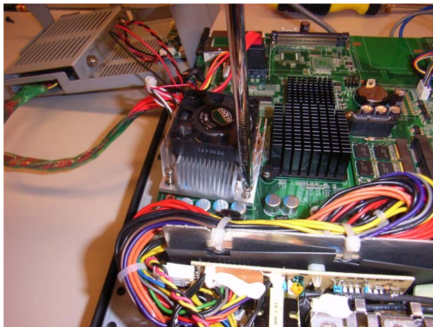
Figure 4.9 Placing the Heatsink and Fan on the CPU and then Fastening
