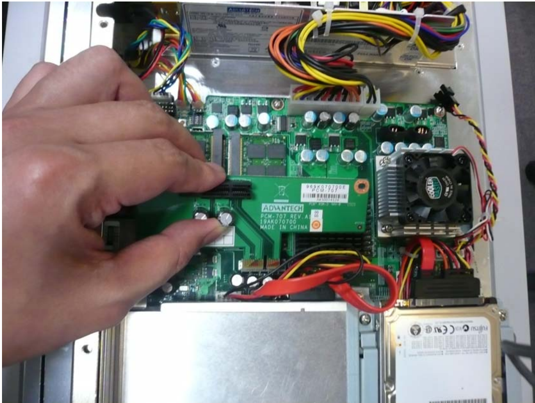
Figure 3.2 PCI & PCI-E Bus Expansion
