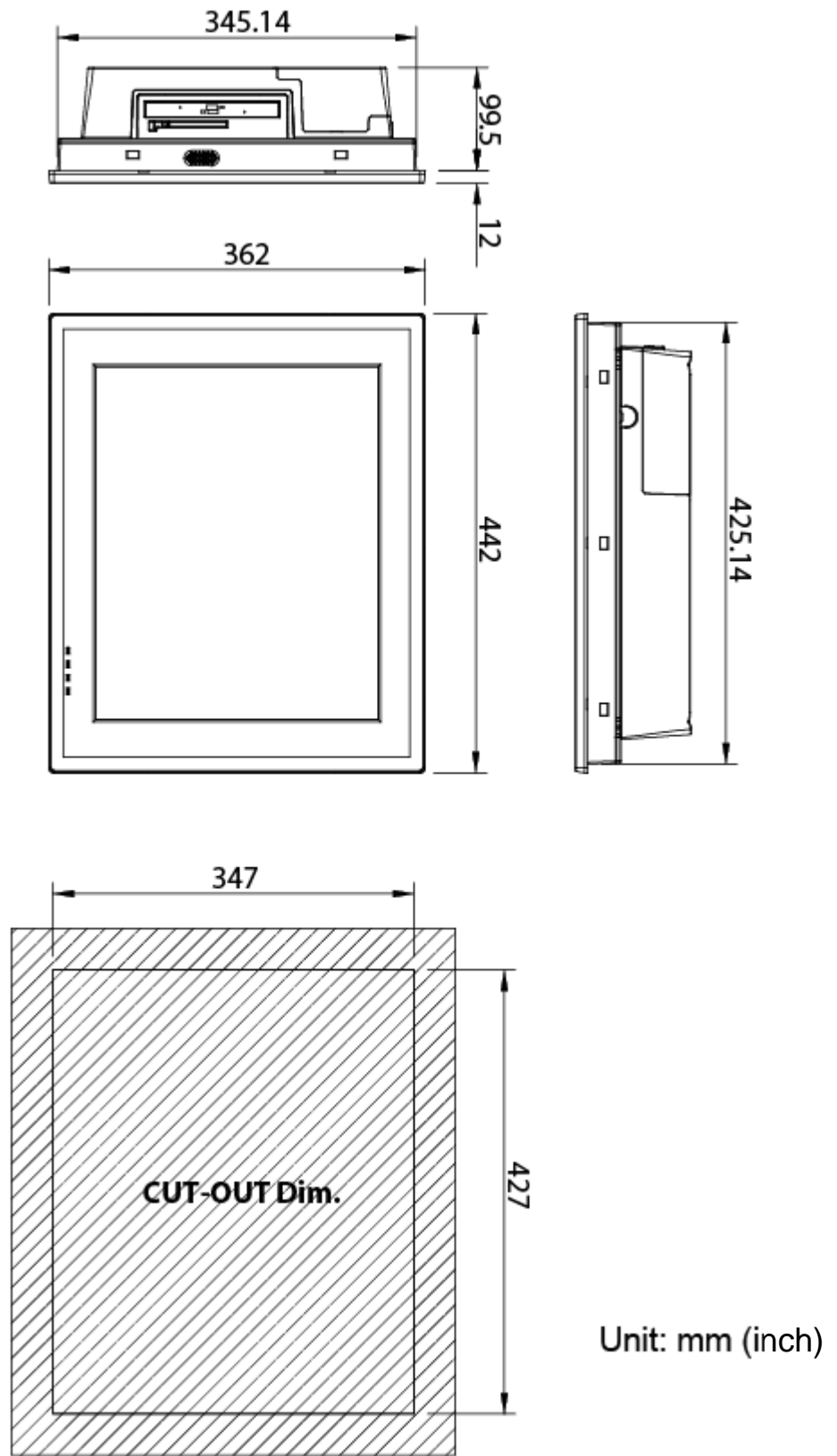
Figure 1.1 Dimensions of PPC-177T
