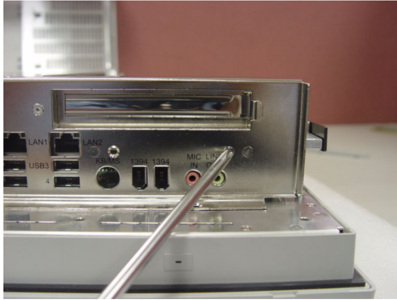
Figure 4.14 I/O Shielding
