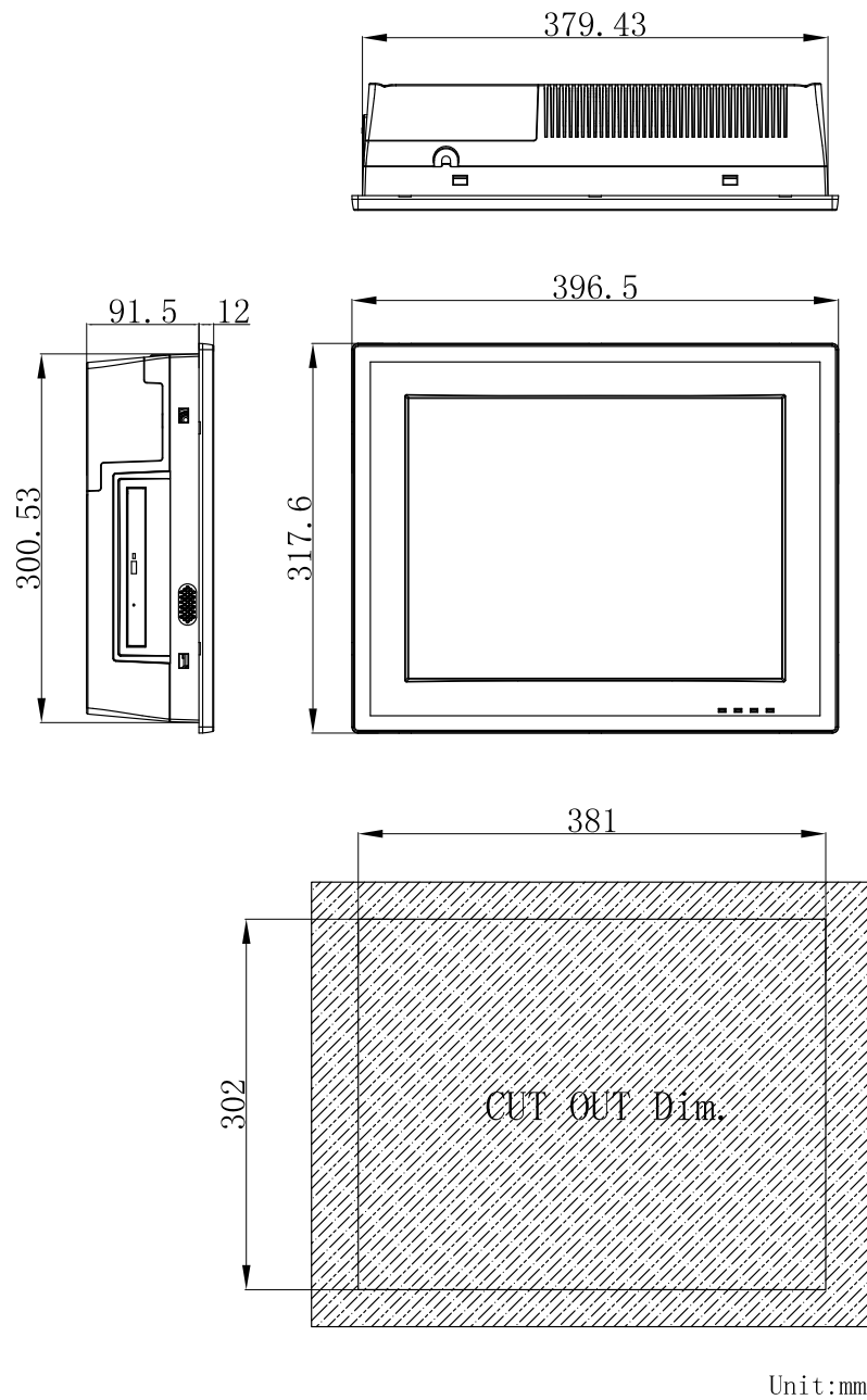
Figure 1.1 Dimensions of PPC-157T
