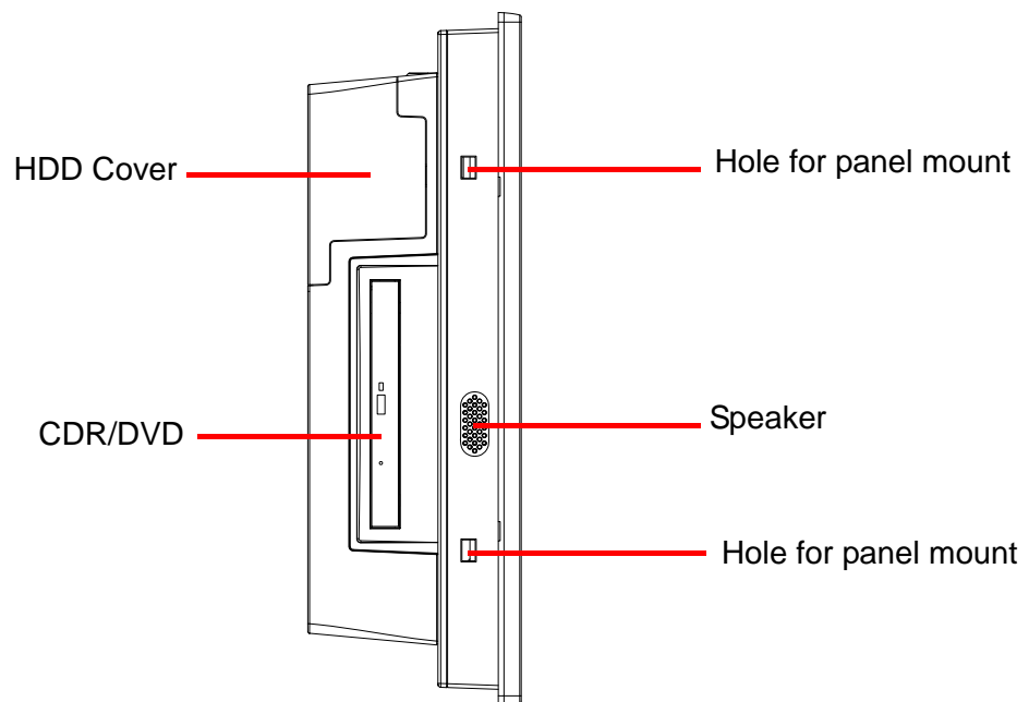
Figure 2.2 Side View of the Panel PC
