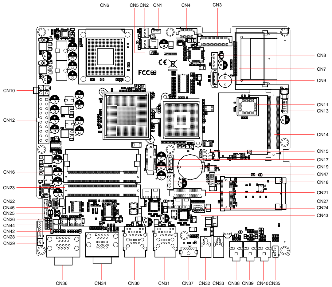
Figure 5.1 Jumpers & Connectors on PPC-157T Motherboard
