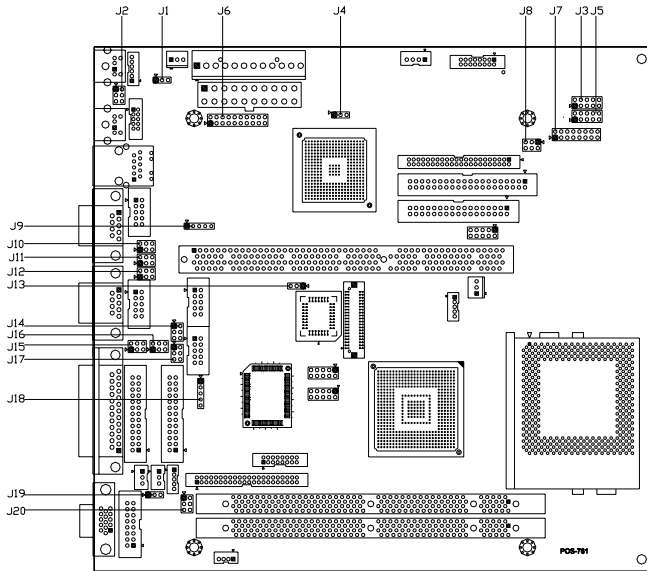
Figure 2.1: Locating Jumpers
