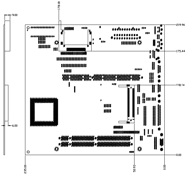
Figure 1.2: Board Dimensions (Solder Side)
