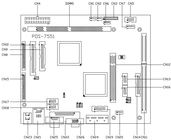
Figure 2-2: Locating connectors
