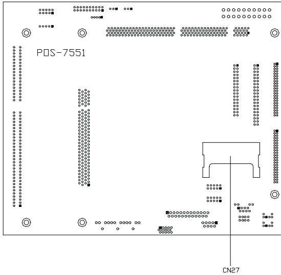
Figure 2-3: Backside connectors
