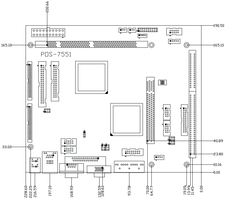
Figure 1-1: Board dimensions (component side)
