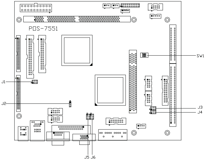
Figure 2-1: Locating jumpers
