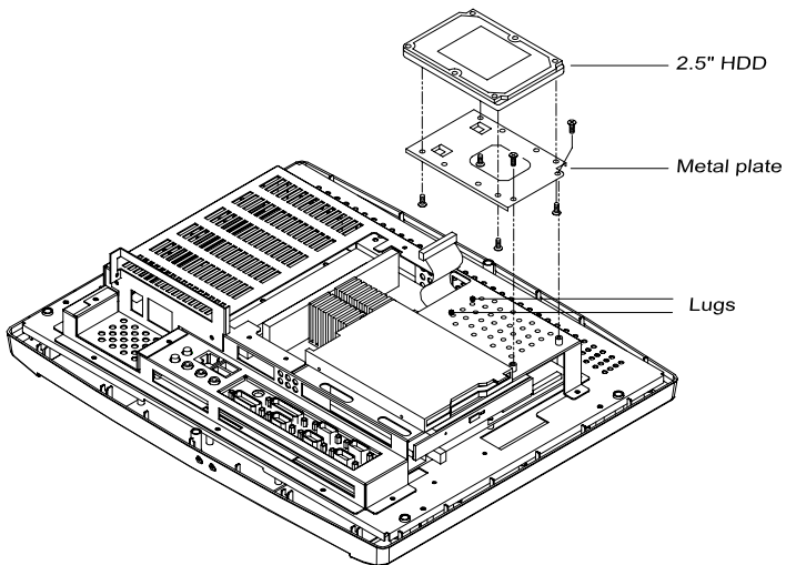
Figure 4.2: Installing the primary 2.5" HDD
