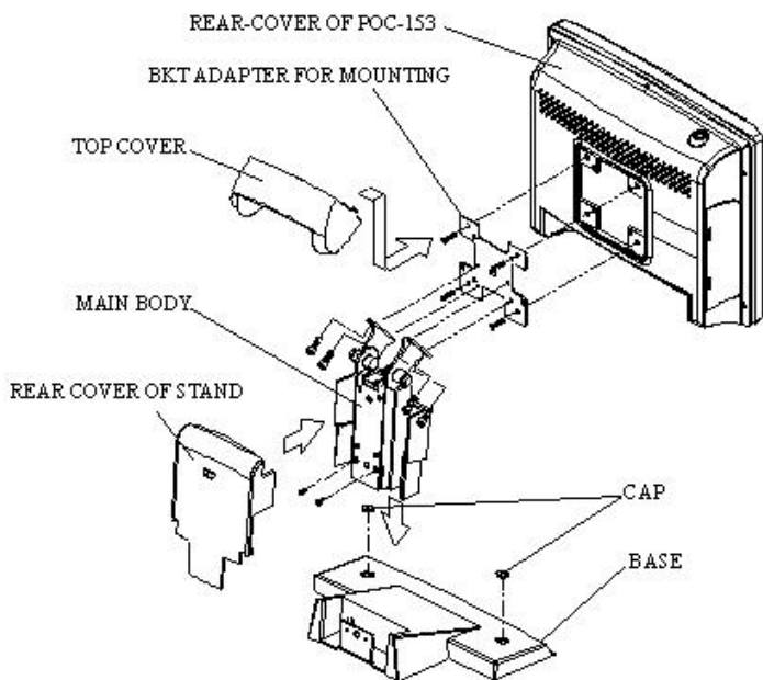
Figure E.1: Desktop stand mounting
