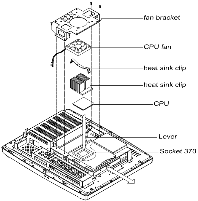
Figure 4.3: Installing the CPU
