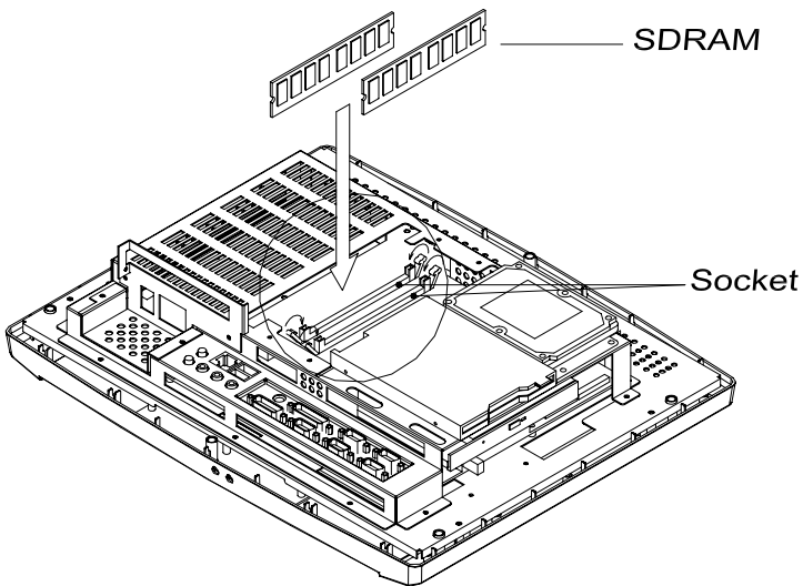
Figure 4.4: Installing SDRAM
