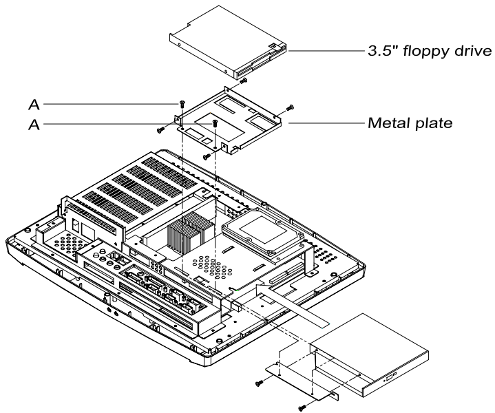
Figure 4.5: Installing FDD and slim CD-ROM drive
