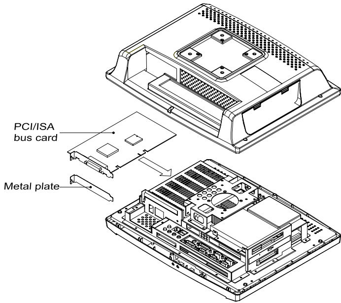
Figure 3.6: PCI/ISA bus expansion
