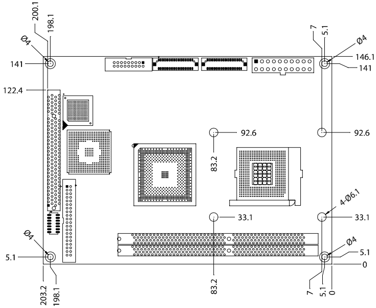
Figure E.1: PCM-9580 Mechanical Drawing (component side)
