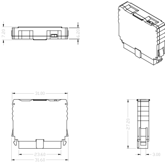
Figure 2.2: Embedded USB Mod. Type I
