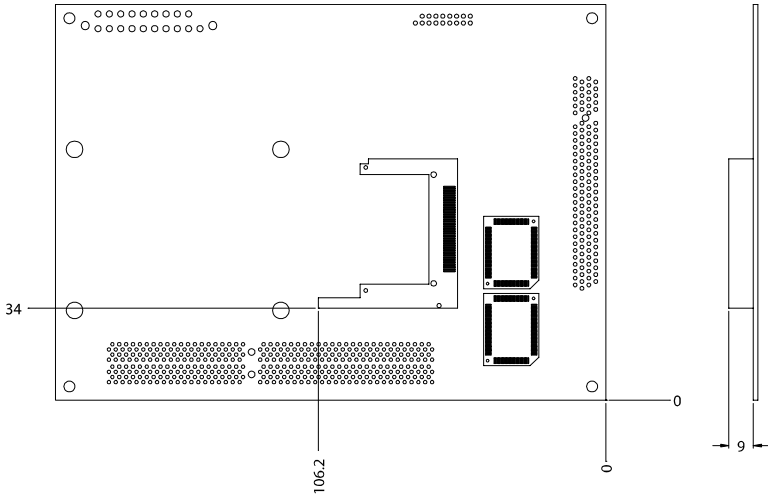
Figure E.2: PCM-9580 Mechanical Drawing (solder side)
