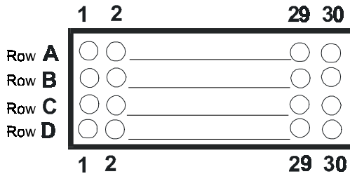
CN18: PC/104-Plus connector (PCI bus) (PCM-9550F/9550FM only)
