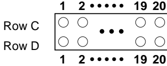
CN18 (ISA bus short side)
