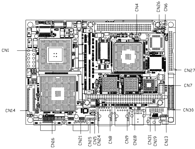
Figure 2.1: Connectors (component side)
