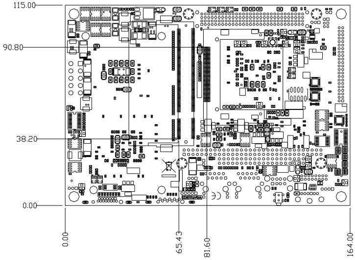
Figure 1.2: Board layout: Dimensions (Solder Side)
