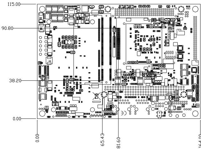
Figure E.2: PCM-4380 Mechanical Drawing (Solder Side)
