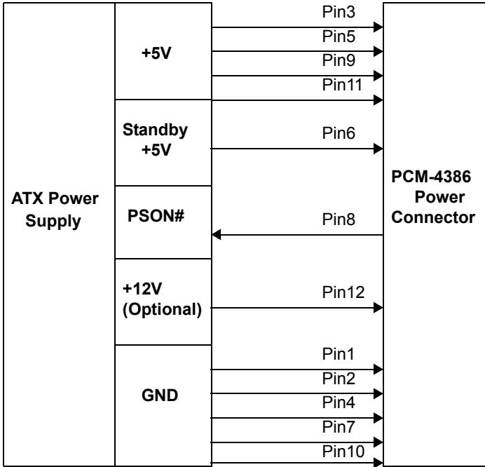
Figure D.1: ATX power supply diagram
