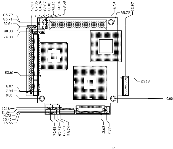
Figure D.1: PCM-3386 Mech Drawing (component side)
