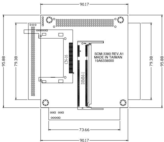
Figure D.2: PCM-3386 Mech Drawing (solder side)
