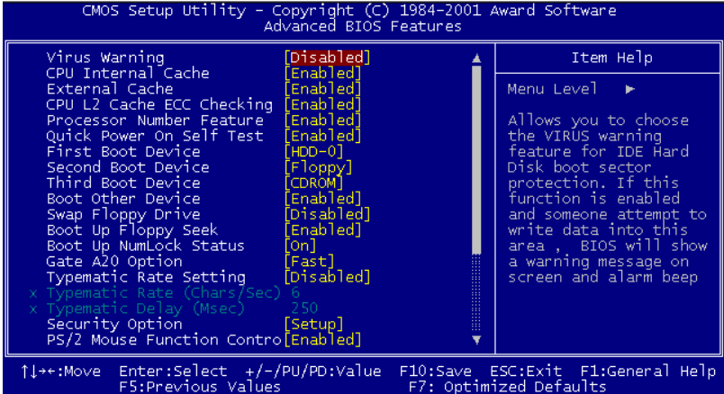
Figure 6.3: Advanced BIOS Features setup
