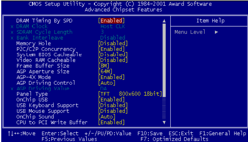
Figure 6.4: Advanced Chipset Features setup
