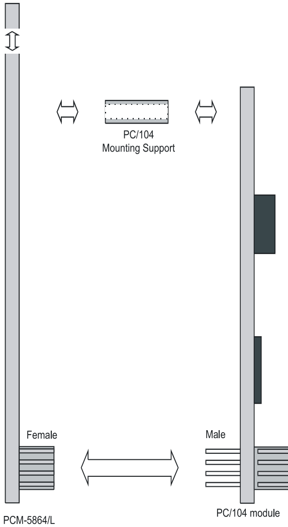
Figure B.1: PC/104 module mounting diagram
