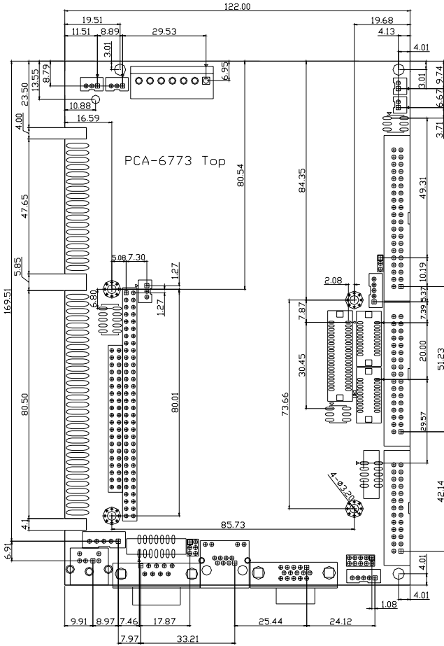
Figure 1.1: Board layout: dimensions (component side)
