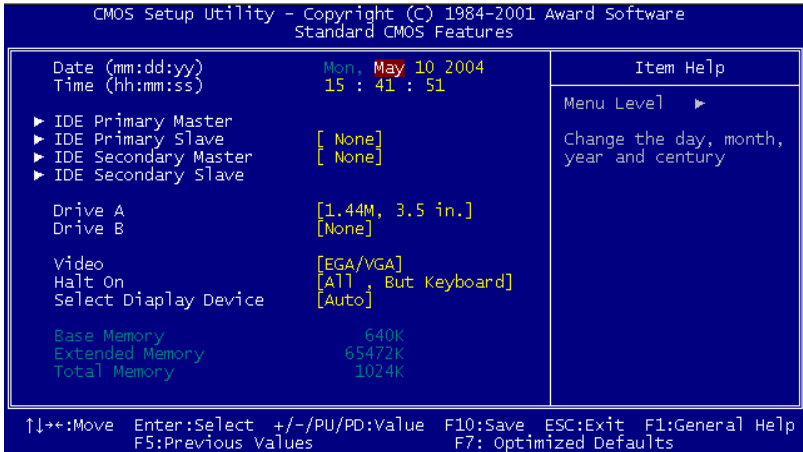
Figure 6.2: CMOS Features setup
