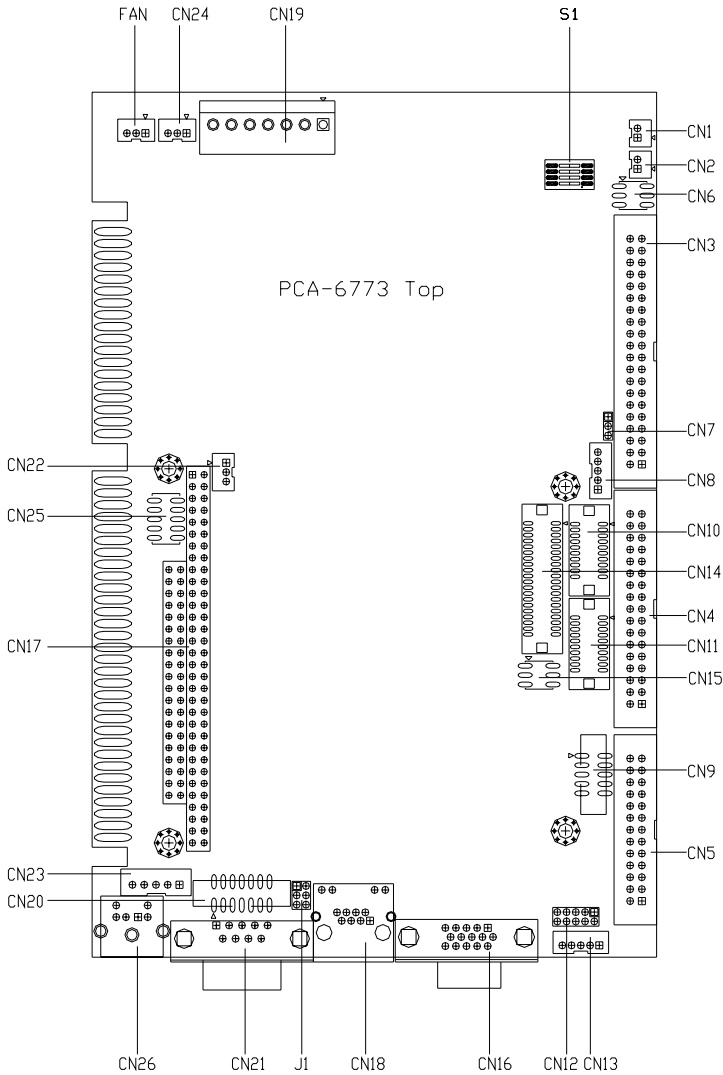
Figure 2.1: Jumper & Connector Locations
