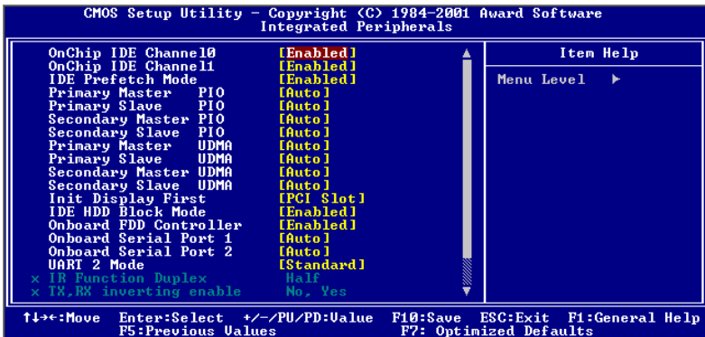
Figure 3-5: Integrated peripherals (1)
