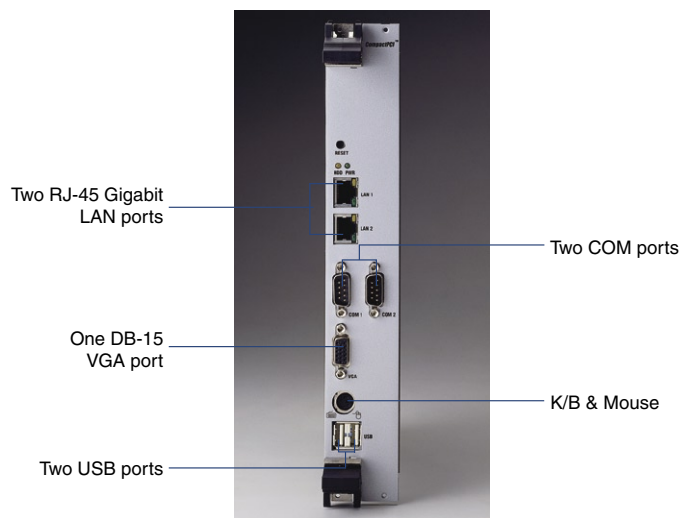
Onboard I/Os of front panel
