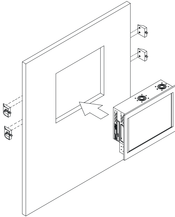
Figure 2-11: Panel mounting
