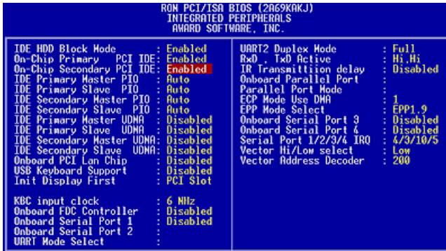
Figure 9-8: Integrated peripherals screen
