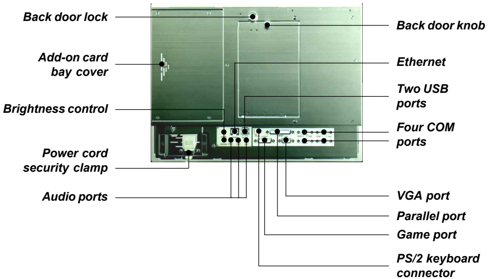
Figure 2-2: Rear view
