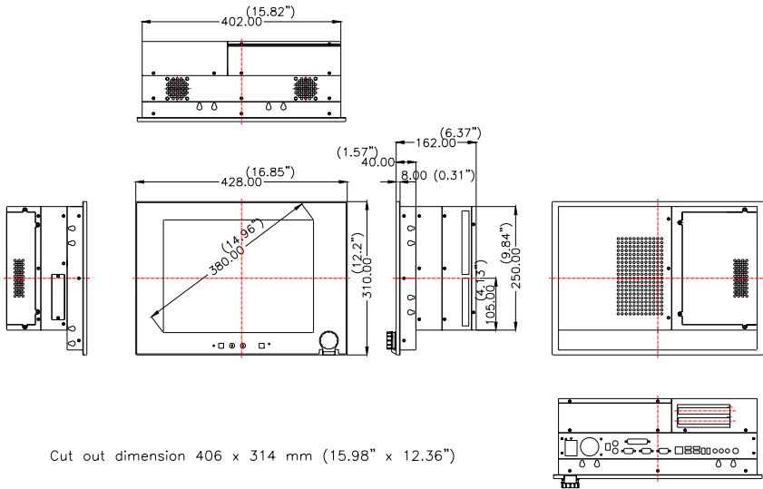
Figure 1.1: IPPC-9151FA Dimensions
