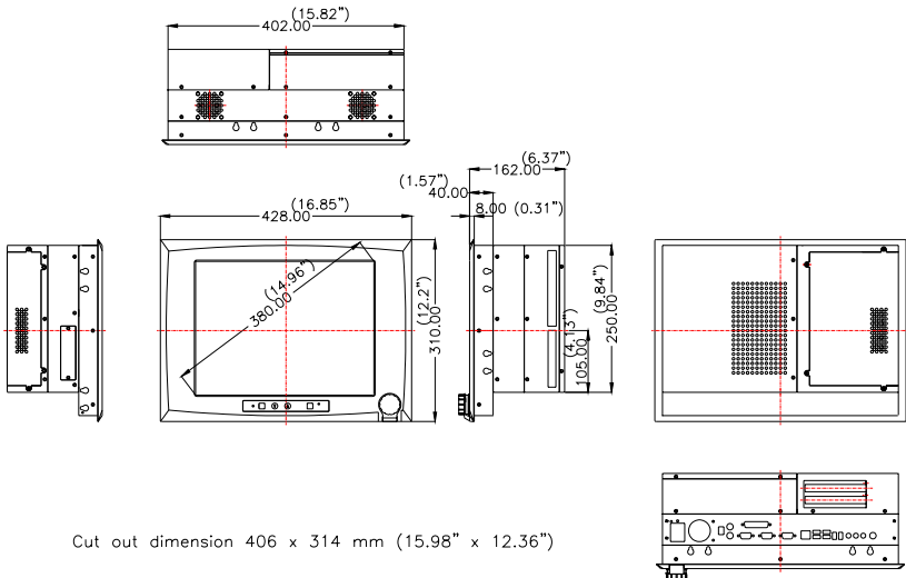
Figure 1.2: IPPC-9151GA Dimensions
