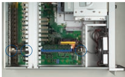
Enhanced anti-vibration mechanical design for full-sized CPU card
