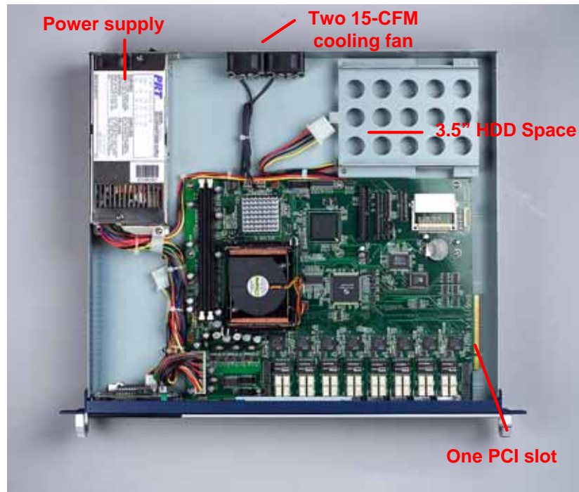
Figure 2-3: Top view of FWA-3180
