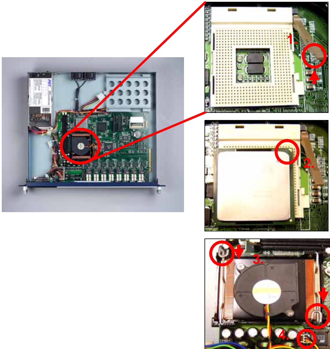
Figure 2-4: Installing Central Processing Unit steps
