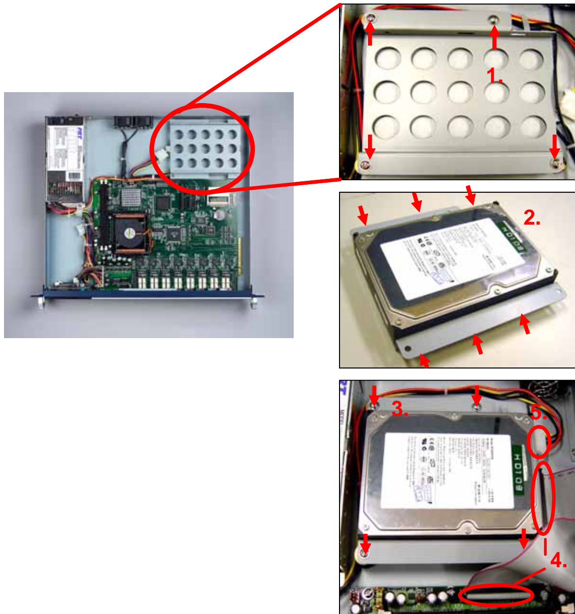
Figure 2-6: Installing Hard Disk Drive steps
