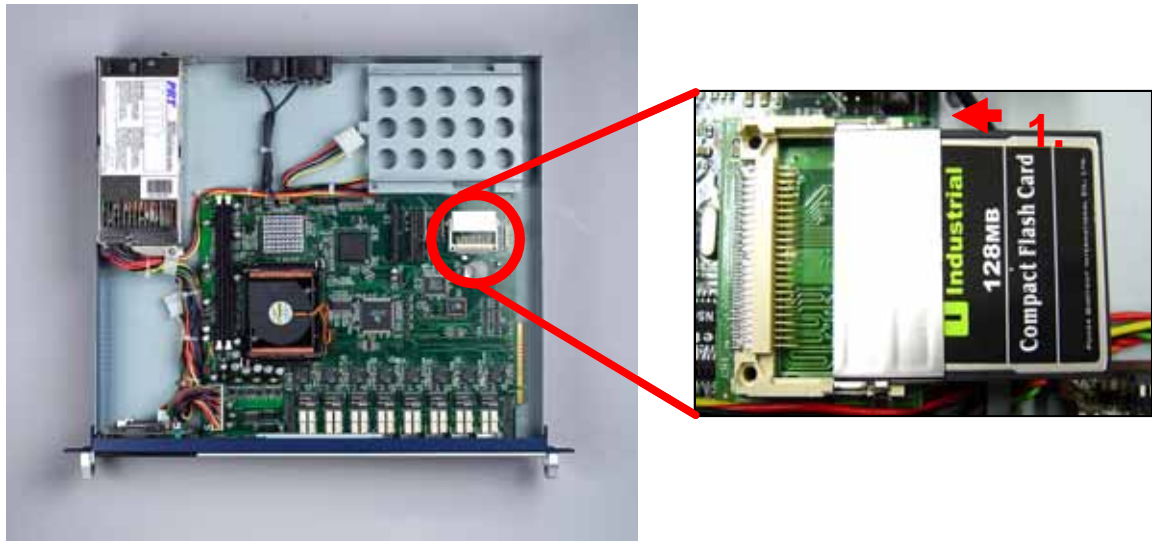
Figure 2-7: Installing Compact Flash steps
