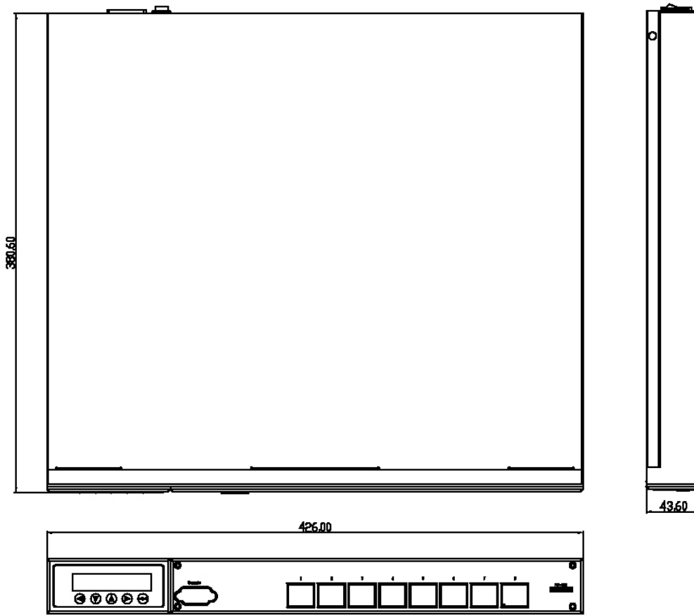
Figure 1-1: FWA-3180 dimensions.
