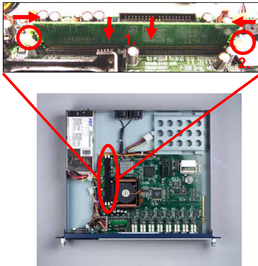
Figure 2-5: Installing Memory Module steps
