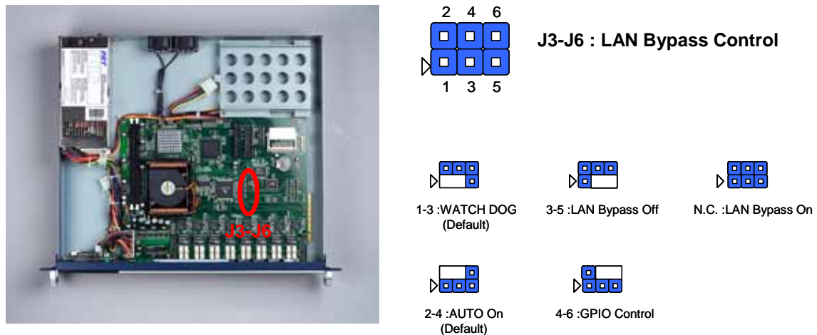
Figure 2-9: LAN Bypass function jumps
