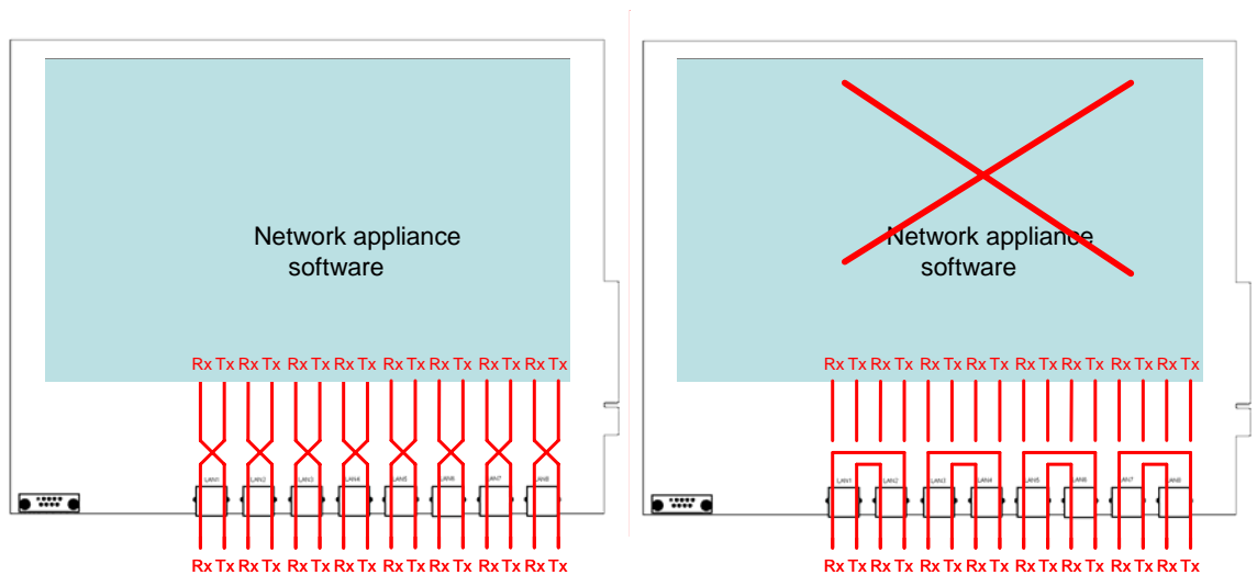
Figure 2-8: The illustration of LAN Bypass function
