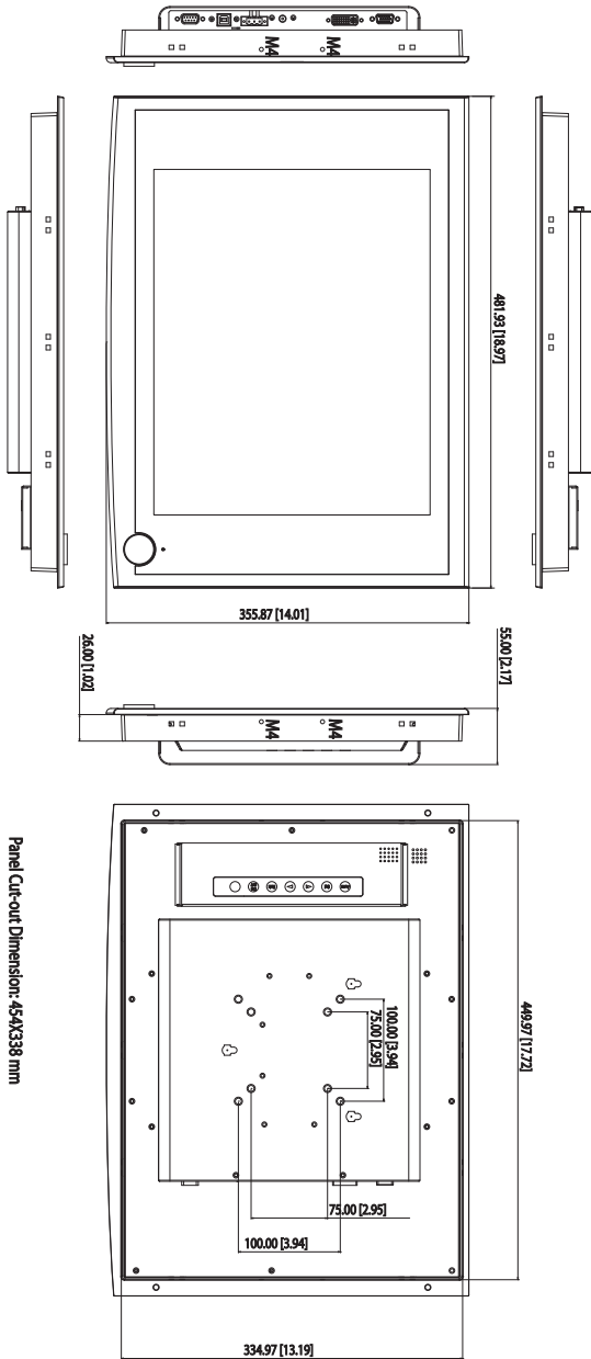
Figure 1.1: FPM-5171G Dimensions
