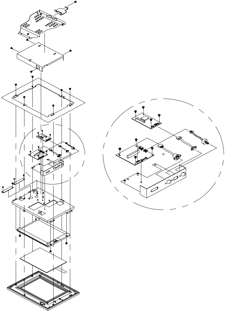
Figure 2-3: Exploded diagram
