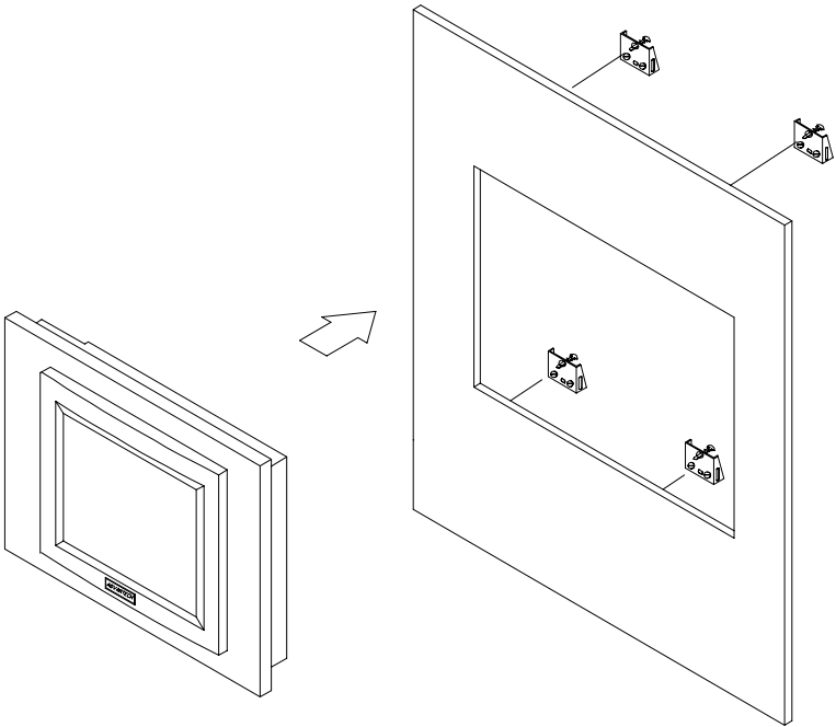
Figure 2-2: Panel mounting
