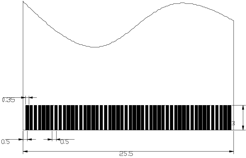
Figure A-3: FPC cable layout
