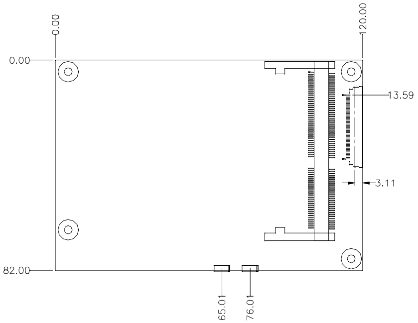
Figure 1-2: Board layout: dimensions (solder side)
