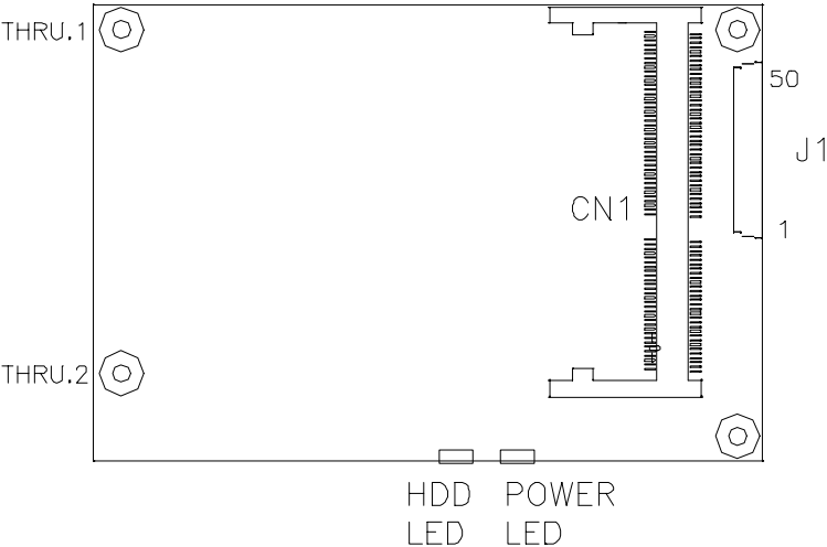
Figure 2-2: Board layout: connector locations (solder side)
