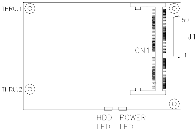
Figure A-2: Board layout: location of Pin 1 of J1 (solder side)
