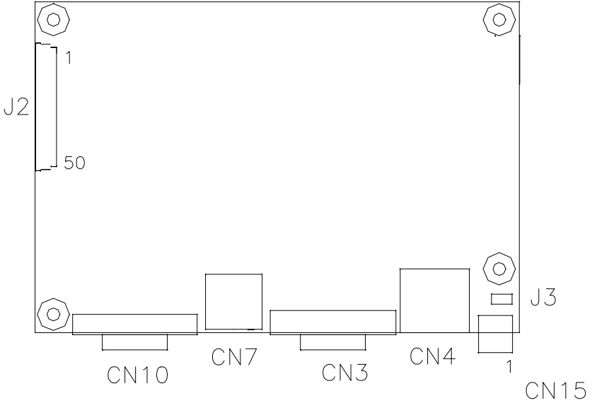
Figure A-1: Board layout: location of Pin 1 of J2 (component side)
