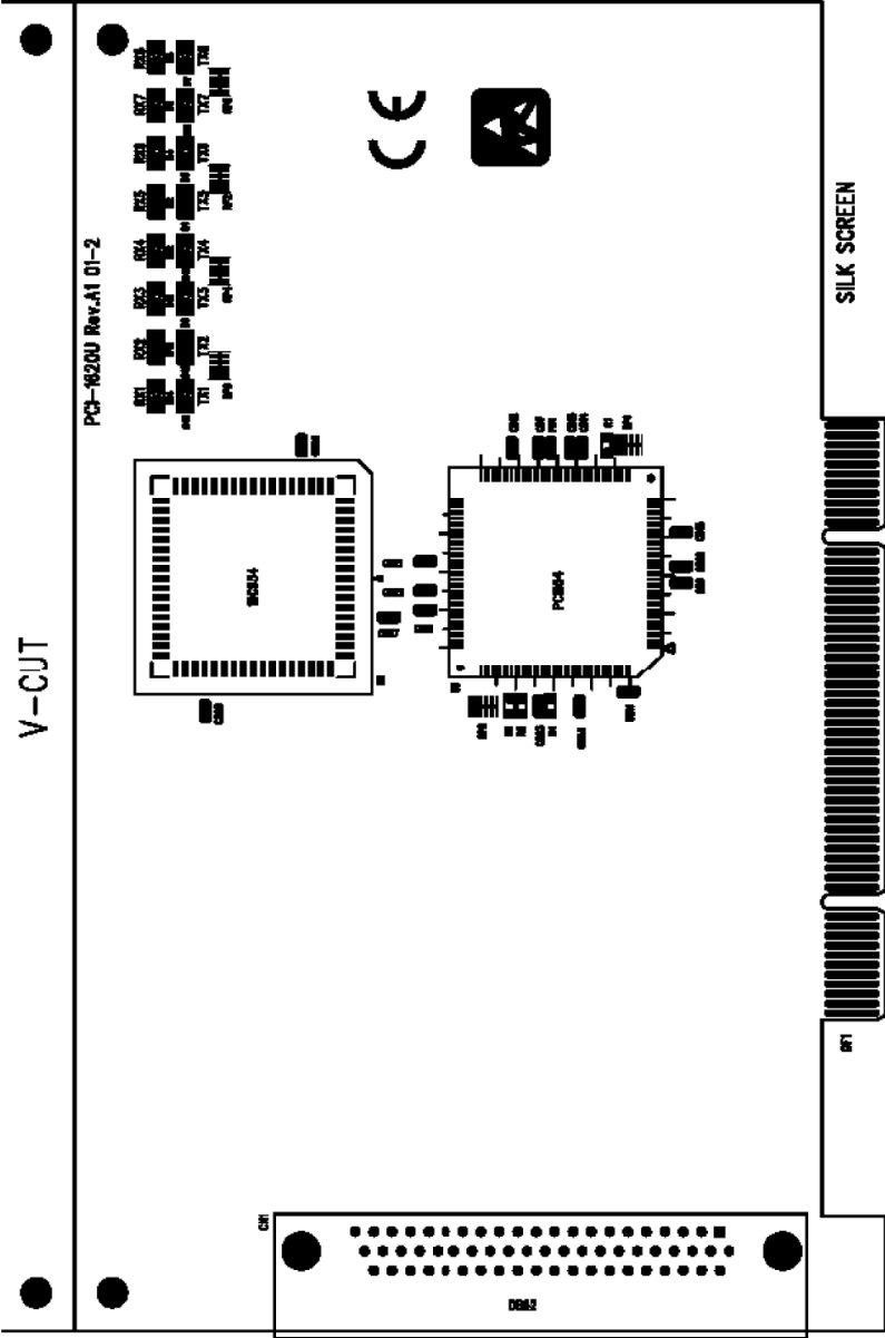
Figure 2.17: PCI-1620AU/U Silk Screen
