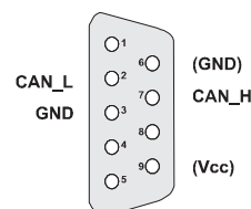
Control Area Network
