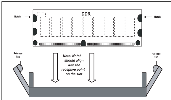
Figure 2-2. Installing and Removing DIMMs
