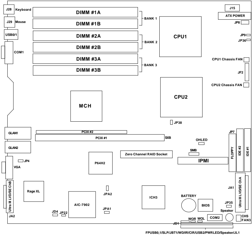
Figure 1-2. Layout* (not drawn to scale)
