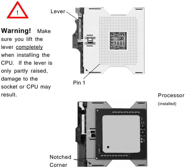
Figure 2-1. PGA604 Socket: Empty and with Processor Installed
