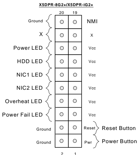
Figure 2-4. JF2 Header Pins
