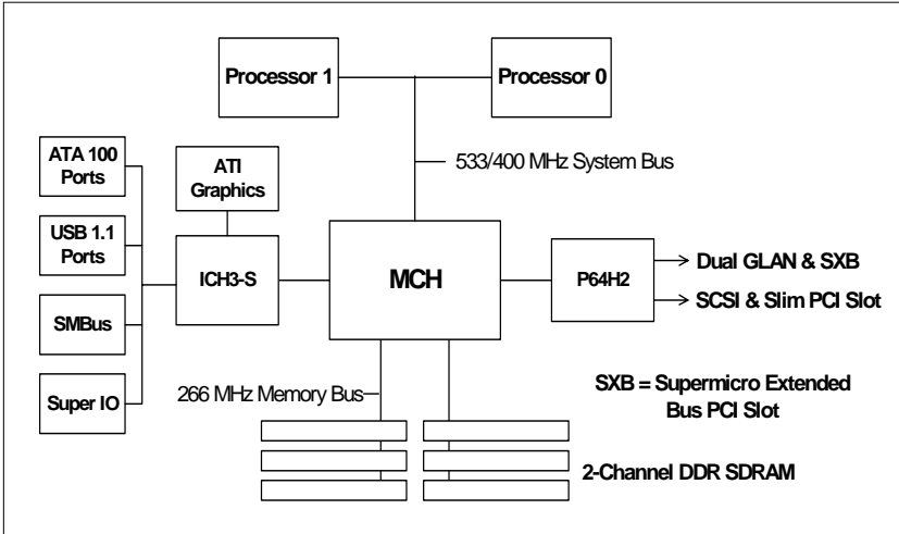
Figure 1-3. Intel E7501 Chipset: System Block Diagram
