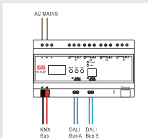
KNX gateway
