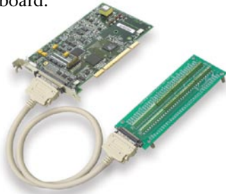
DaqBoard/3000 attached to a TB-100 terminal board
