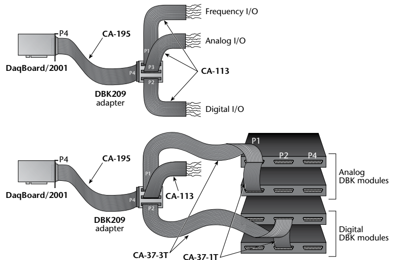
The DBK209 adapter with analog and digital DBK signal conditioning and expansion modules
