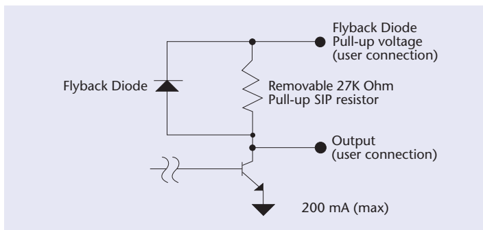
Option HVCX1 high current/voltage output
