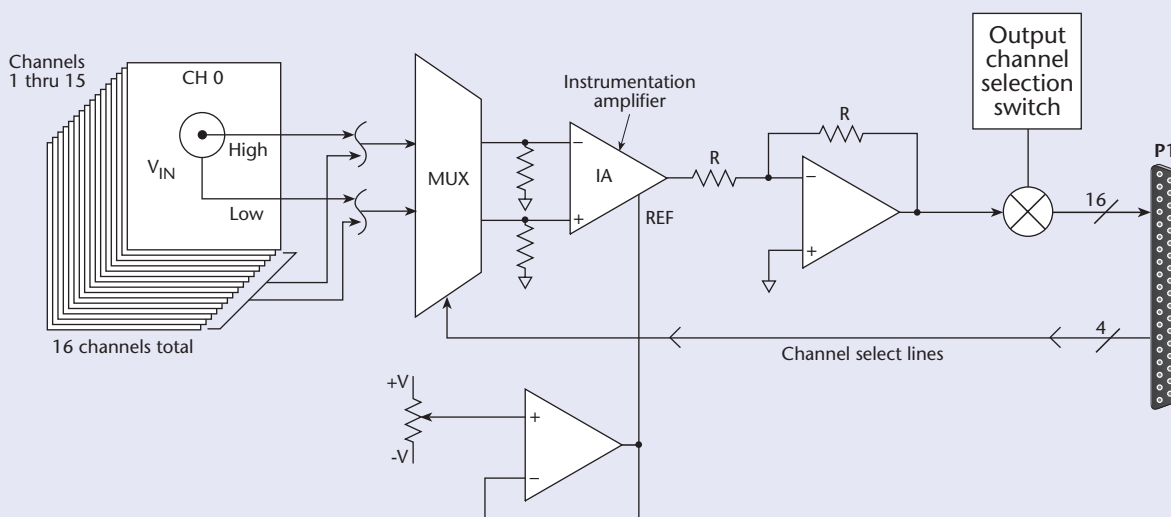
DBK85 Differential Voltage Input Module Block Diagram
