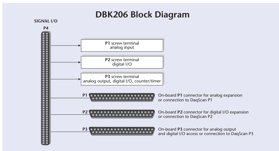
The DBK206 provides removable screw-terminal connectors for DaqBoard/2000 series I/O
