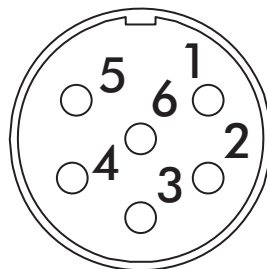
Figure 2.7 Standard M23 6-Pin Male DC Power Input Connector
