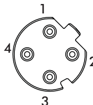
Figure 2.9 10/100BaseT(X) Pin Assignment
