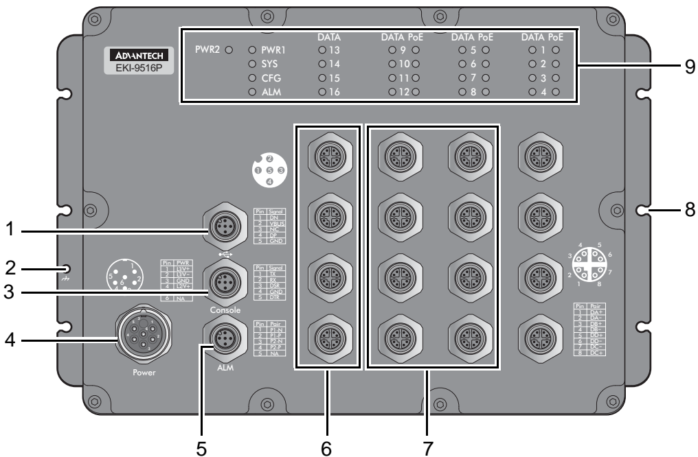
Figure 1.2 Front View
