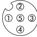
Figure 2.12 M12 Console Pin Assignment
