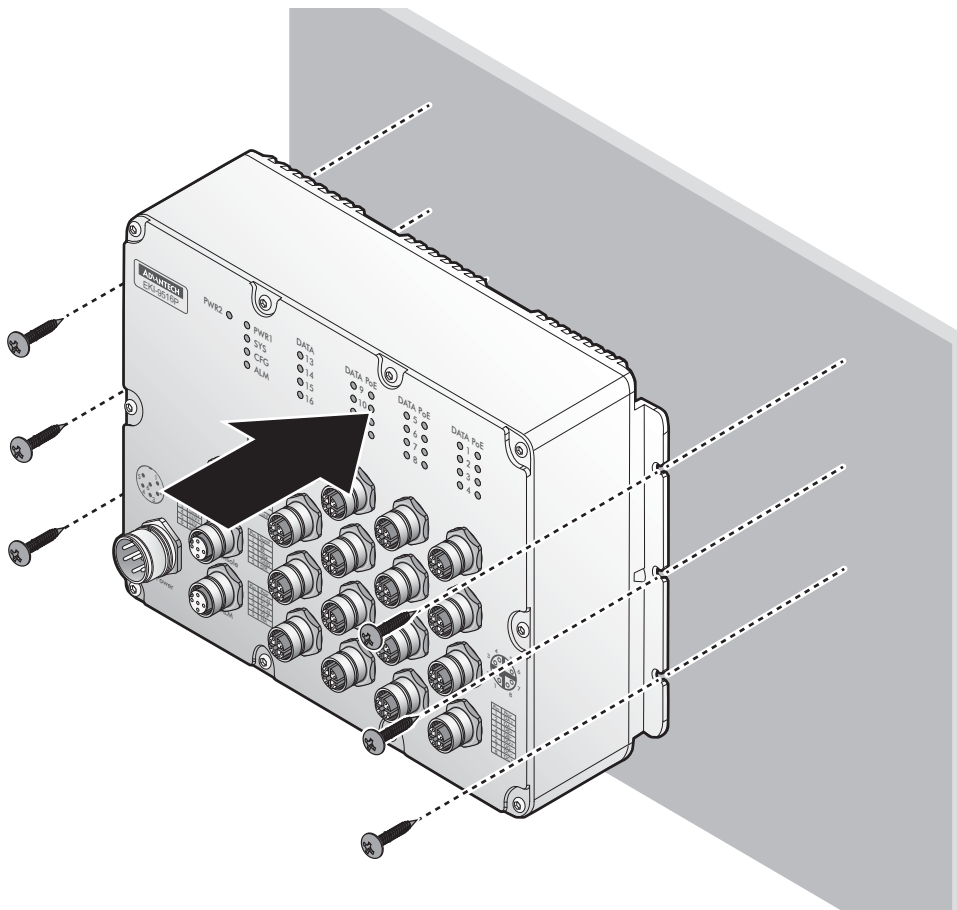
Figure 2.2 Switch Installation
