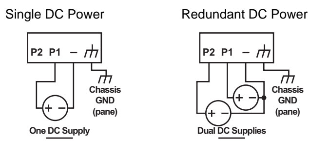
Figure 2.3 Power Wiring for EKI-9500 Series
