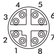
Figure 2.8 10/100/1000BaseT(X) Pin Assignment
