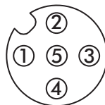
Figure 2.11 M12 Console Pin Assignment
