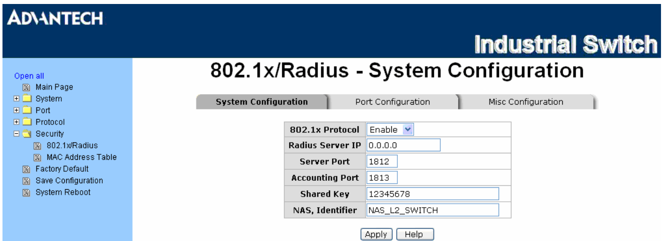
Figure 3.48: 802.1x/Radius System Configuration interface
