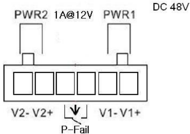
Figure 2.8: Pin Assignment of the Power Connector
