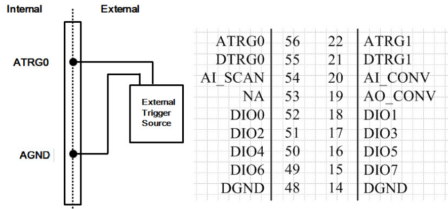
Figure 3.12 External Analog Trigger Source Connection
