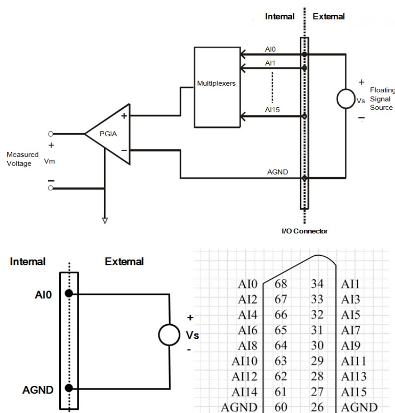
Figure 3.3 Single-ended input channel connections
