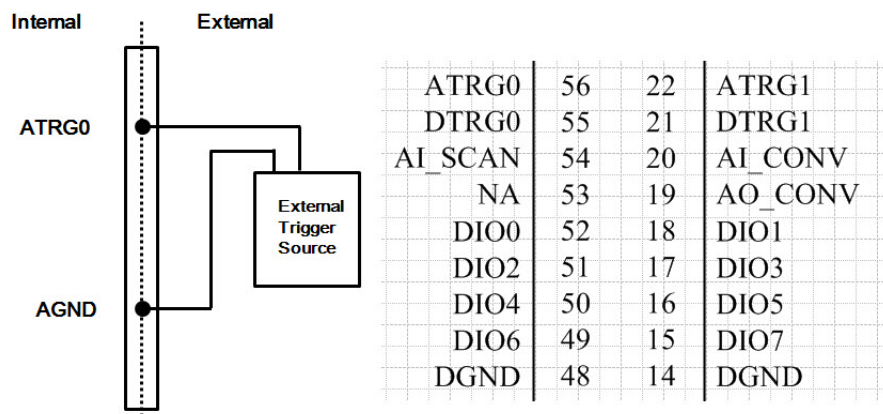
Figure 3.8 External Analog Trigger Source Connection
