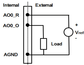
Figure 3.9 Analog Output Connections
