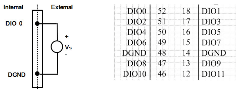
Figure 3.14 Wet signal connection of digital input
