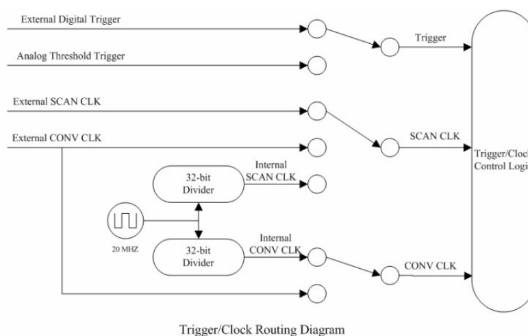
Trigger/Clock Routing Diagram
