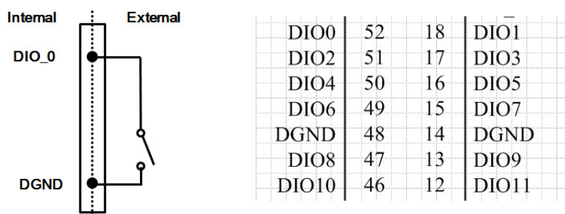
Figure 3.15 Dry signal connection of digital input
