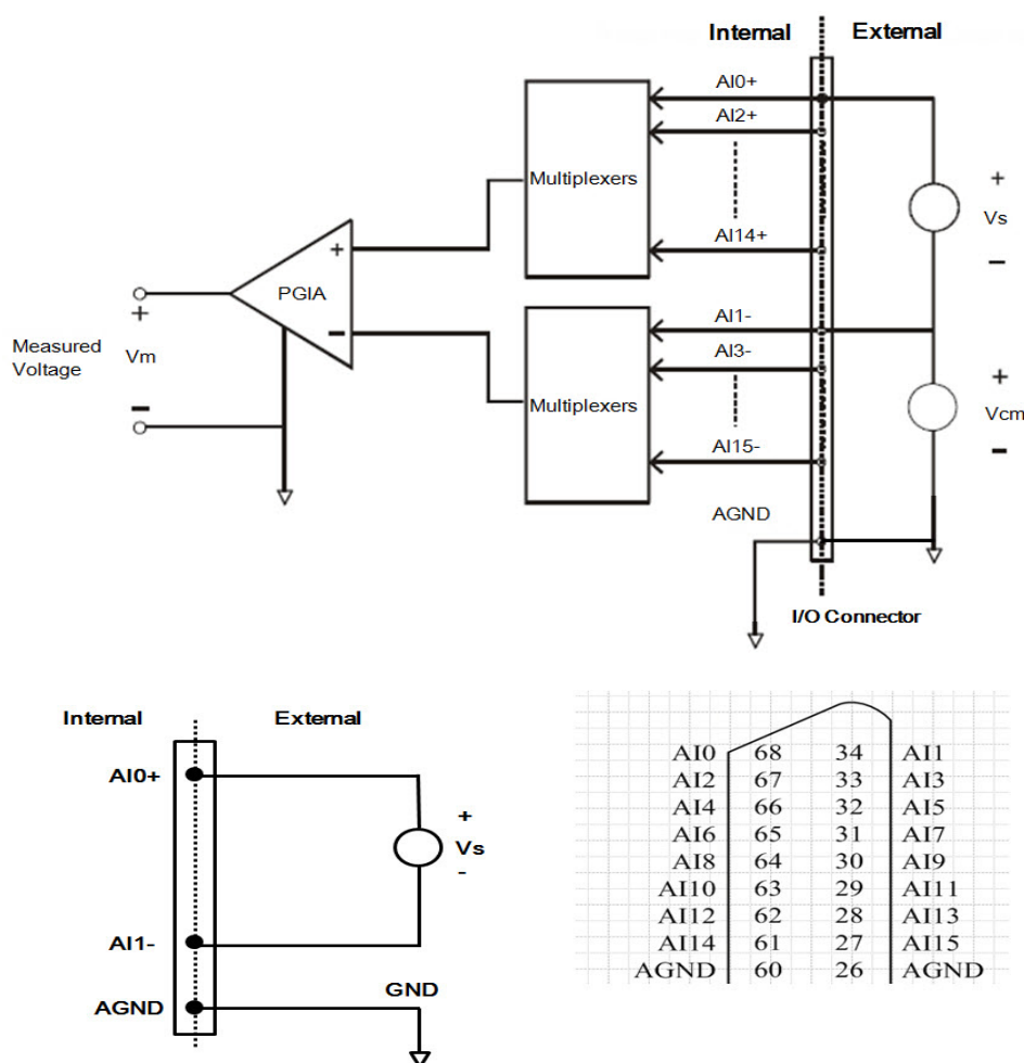
Figure 3.4 Differential input channel connections
