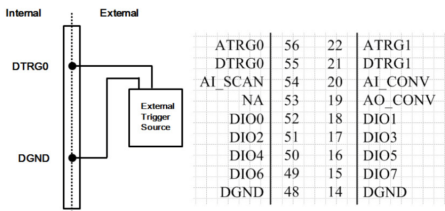
Figure 3.11 External Digital Trigger Source Connection
