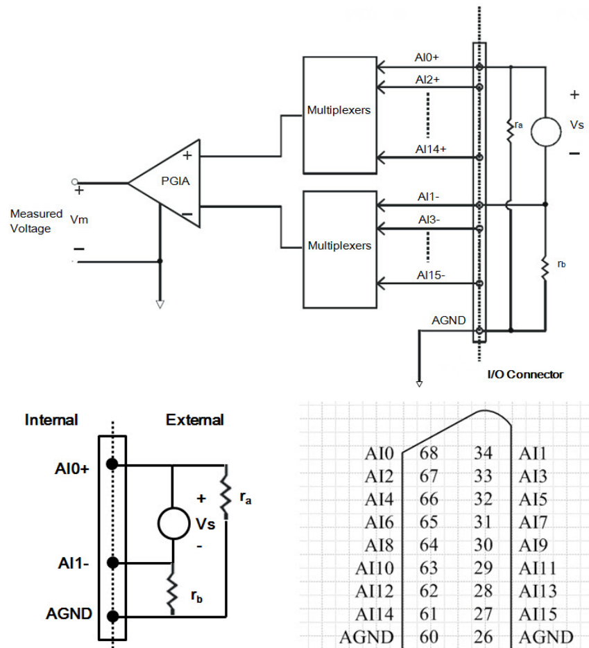
Figure 3.5 Differential input channel connection - floating signal source
