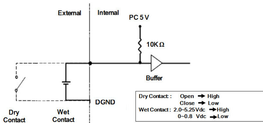
Figure 3.13 Wet and Dry contacts
