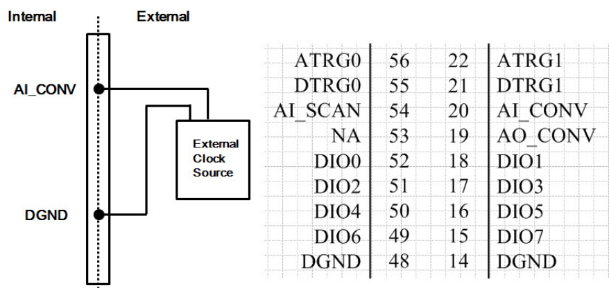
Figure 3.6 External Clock Source Connection
