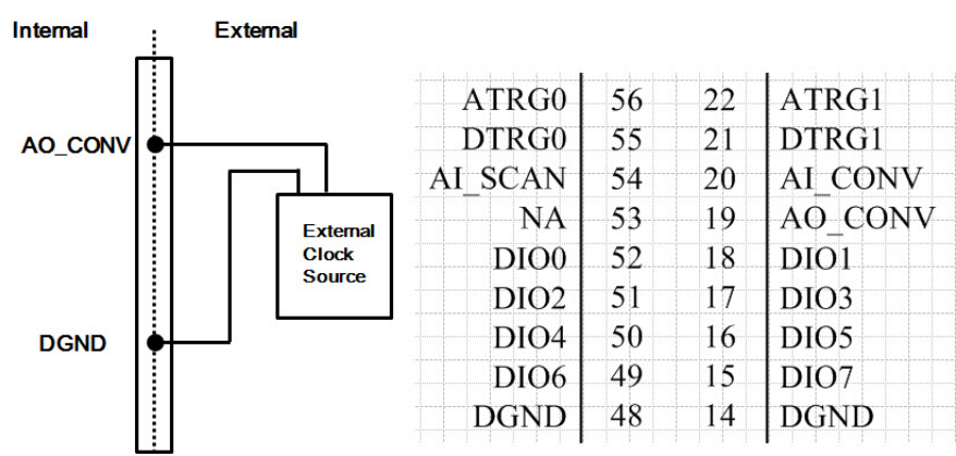
Figure 3.10 External Clock Source Connection
