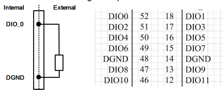
Figure 3.16 Digital Output Channel Connections
