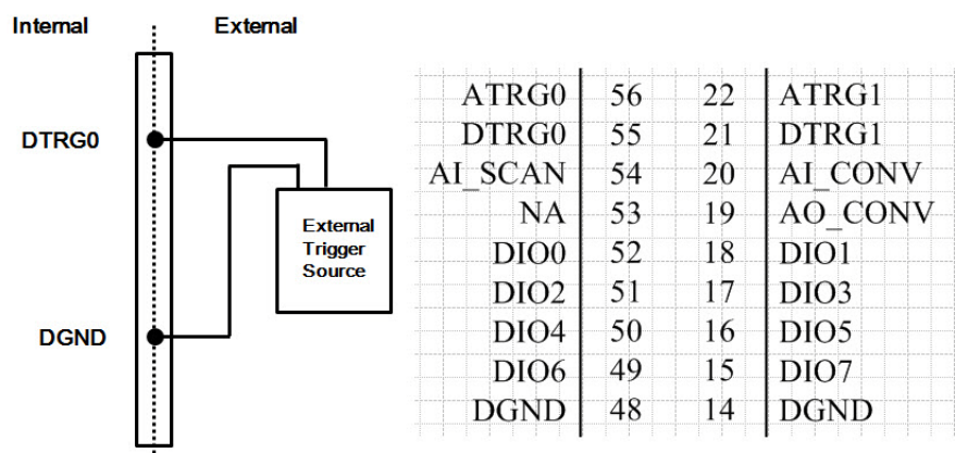
Figure 3.7 External Digital Trigger Source Connection
