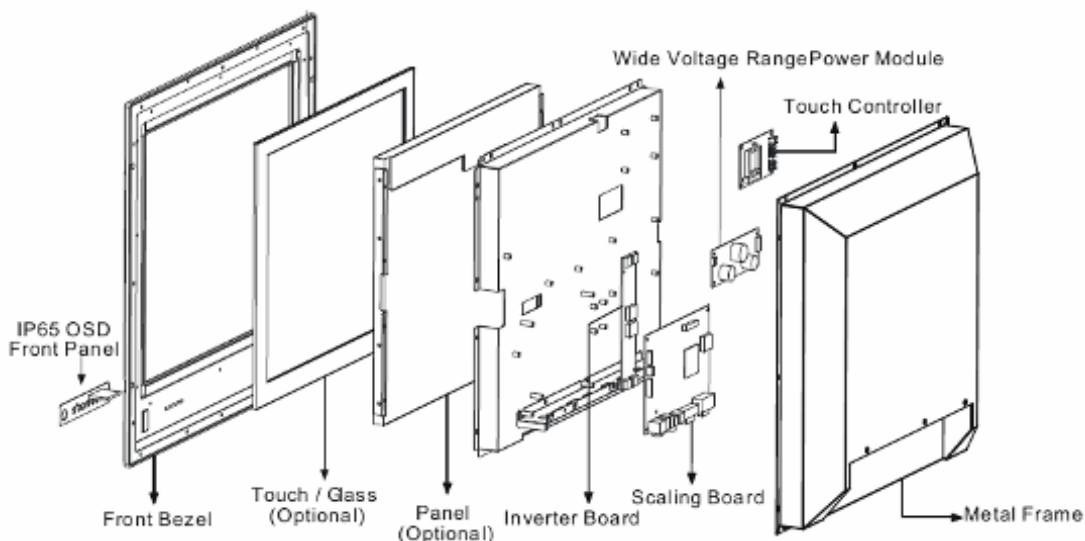
Figure 1.1 Basic Construction
