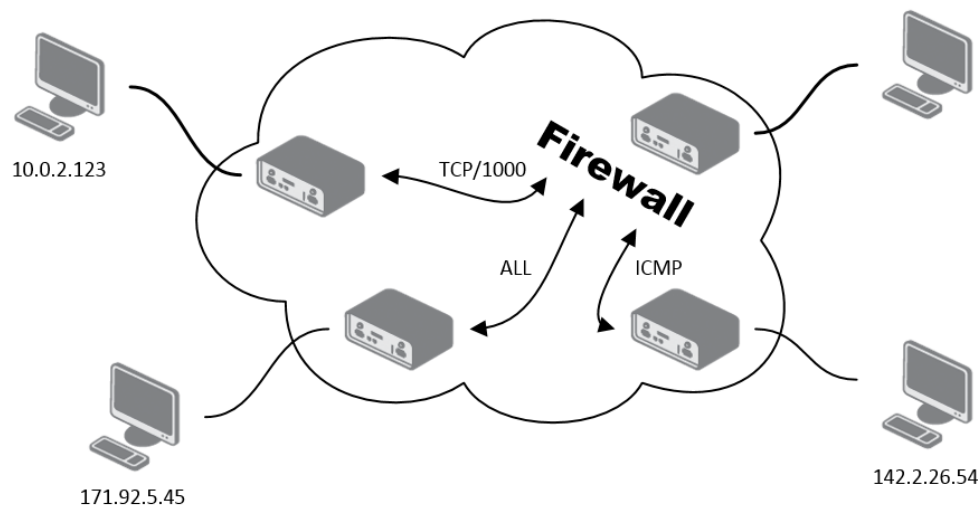
Figure 32: Topology for the IPv4 Firewall Configuration Example
