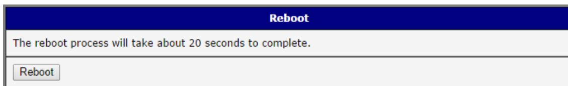
Figure 85: Reboot
