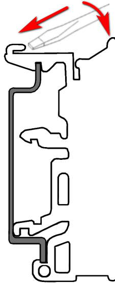
Figure 20: Removing from the DIN rail
