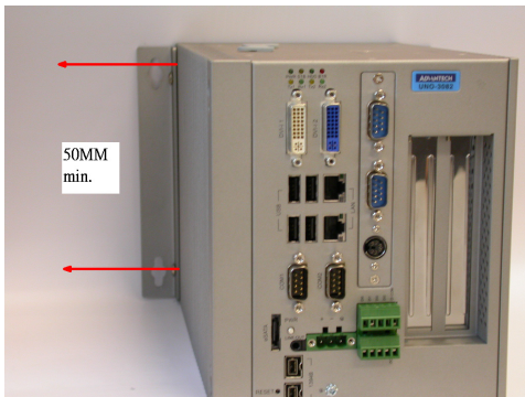
Figure 5: Reserve Space After Panel/Wall Installation
