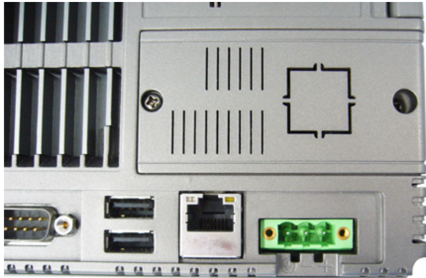
Figure 2.4 Power Receptor & Button Pin Assignment
