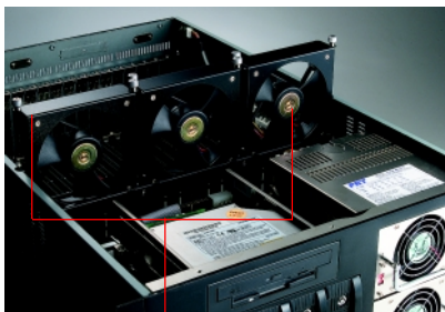
Three 114-CFM hot-swap cooling fans
