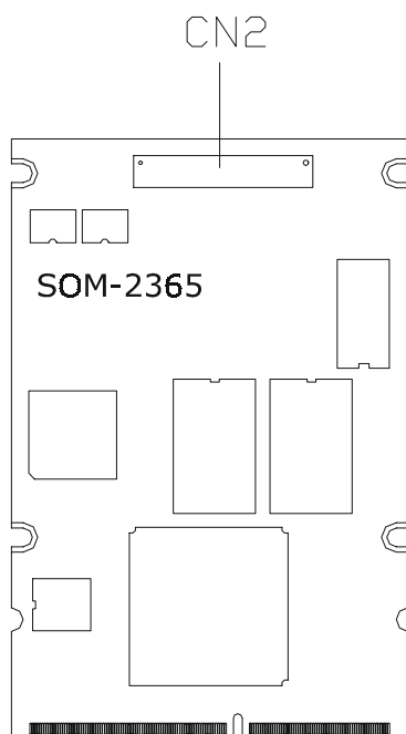
Figure 2.2: Solder side connectors
