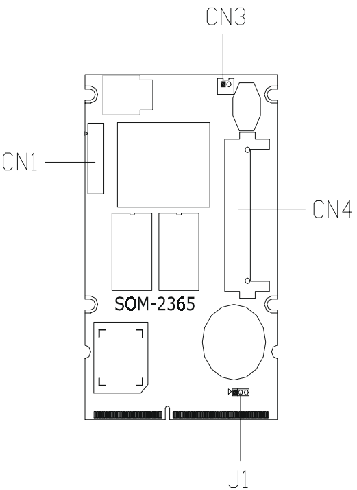
Figure 2.1: Jumper/connector locations
