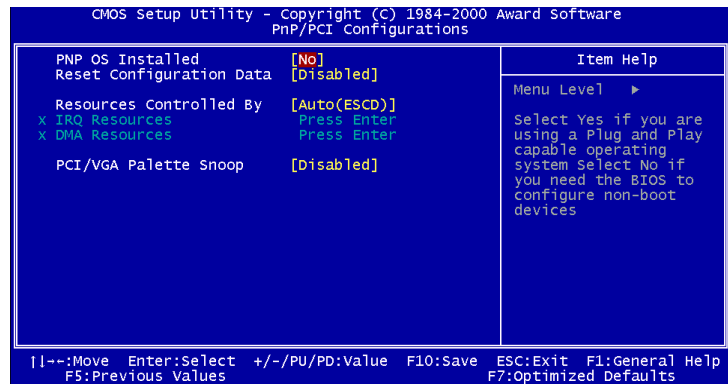
Figure 3.6: PnP/PCI configuration
