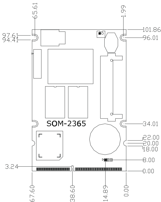
Figure 1.1: Board layout: dimensions
