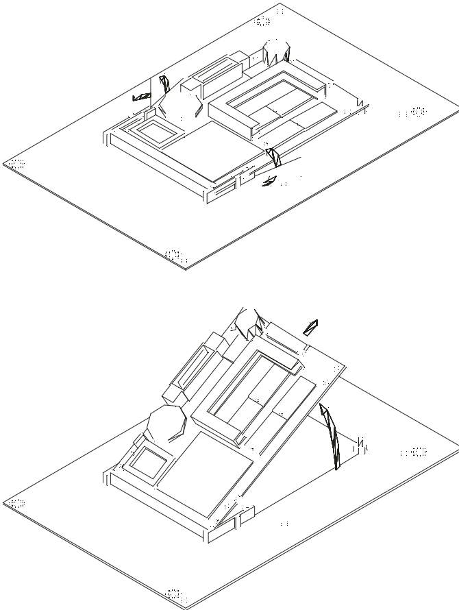
Figure 2.4: SOM-2365 Removal
