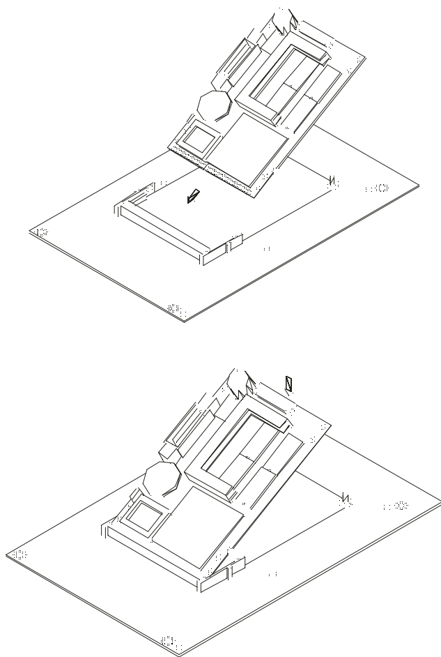
Figure 2.3: Installing the SOM-2365
