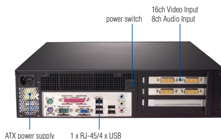
Rear View of PVS-500
