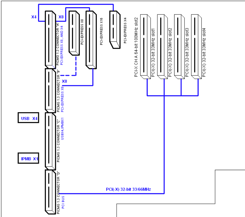
PICMG_v1.3 BACKPLANE
