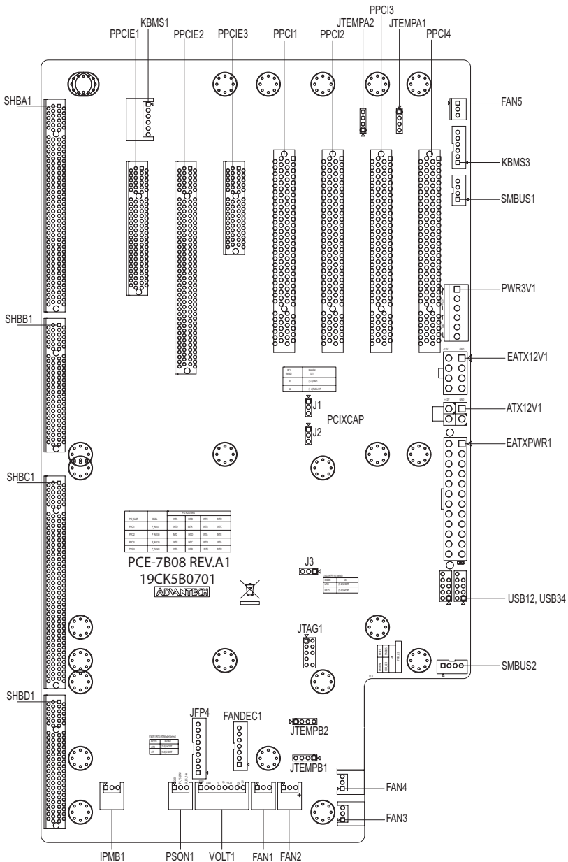
Board Layout: Jumper and Connector Locations
