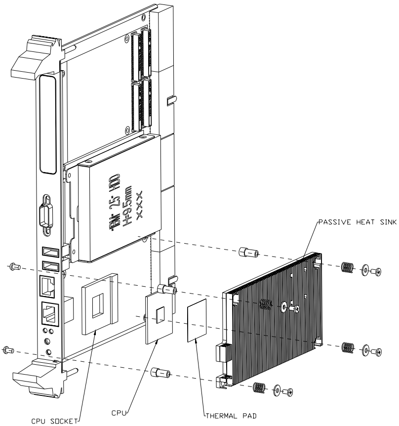
Figure 1.4: Complete assembly, heat sink and HD
